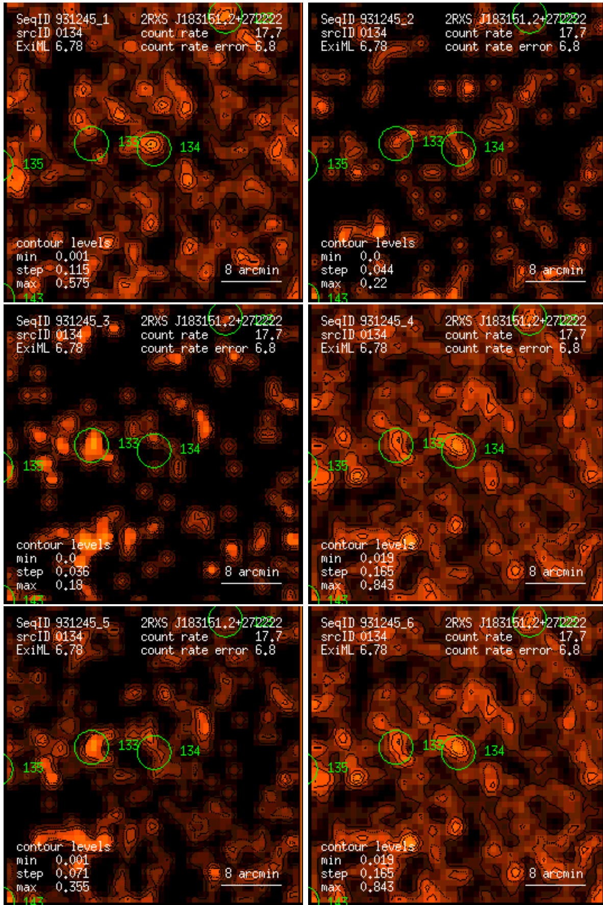
Figure 134: RASS 931245: detection 0134: band rate images, Gaussian filter: (1) PSPC channels 11 – 41, (2) 52 – 90, (3) 91 – 201, (4) 11 – 235, (5) 52 – 201, (6) 11 – 201. Broad band rates in counts/ks. Band rate contour levels in counts/ks/arcmin 2 .
