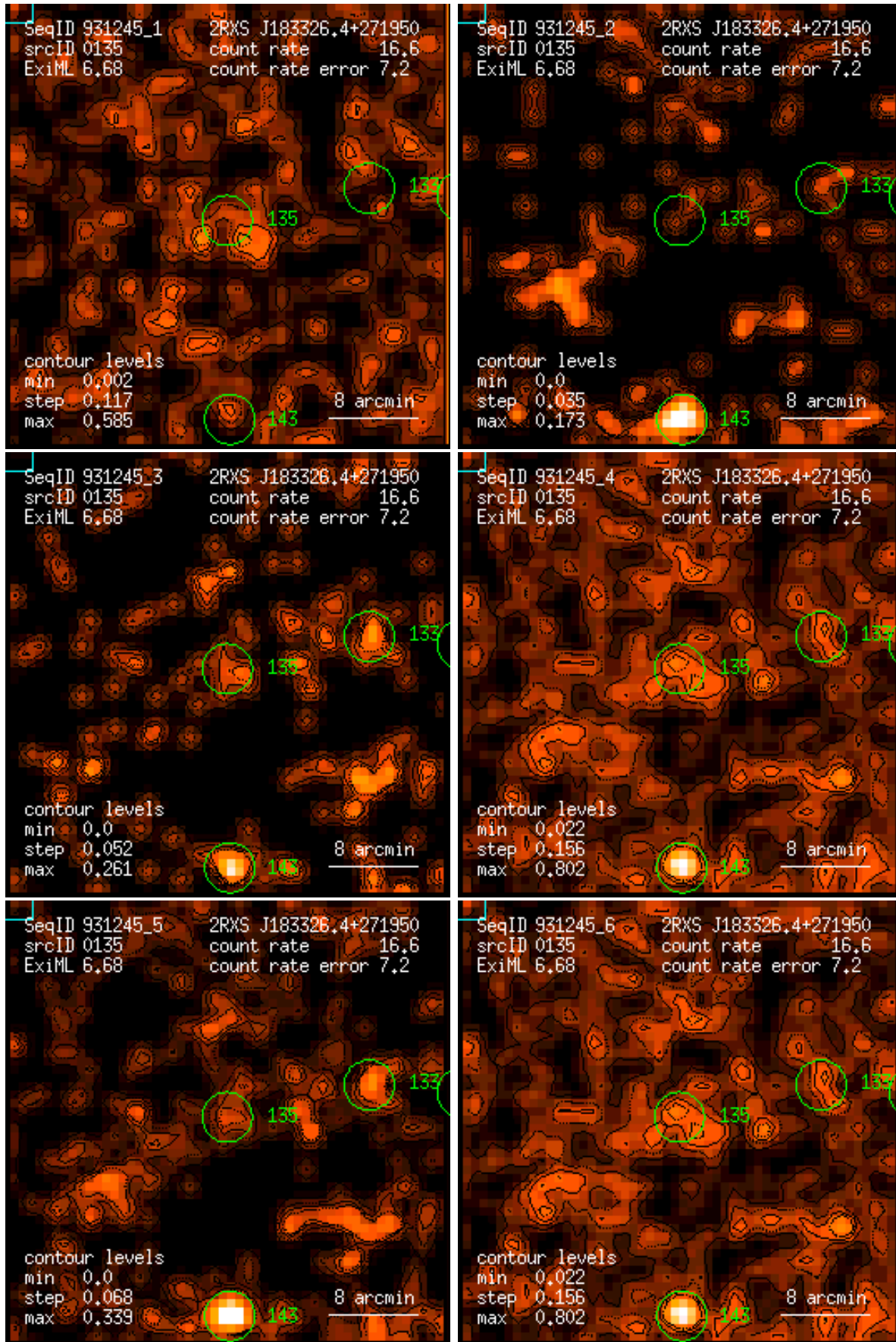
Figure 135: RASS 931245: detection 0135: band rate images, Gaussian filter: (1) PSPC channels 11 – 41, (2) 52 – 90, (3) 91 – 201, (4) 11 – 235, (5) 52 – 201, (6) 11 – 201. Broad band rates in counts/ks. Band rate contour levels in counts/ks/arcmin 2 .
