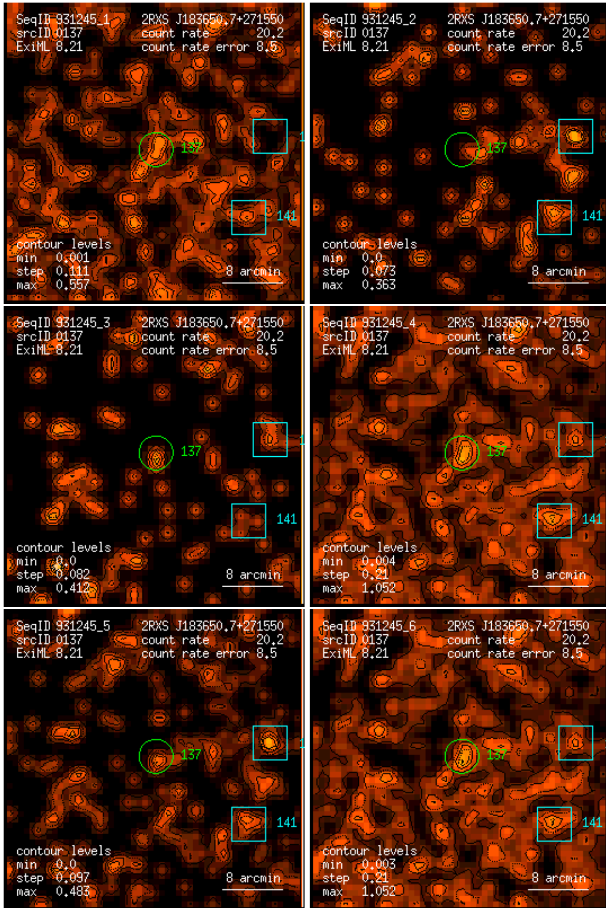
Figure 137: RASS 931245: detection 0137: band rate images, Gaussian filter: (1) PSPC channels 11 – 41, (2) 52 – 90, (3) 91 – 201, (4) 11 – 235, (5) 52 – 201, (6) 11 – 201. Broad band rates in counts/ks. Band rate contour levels in counts/ks/arcmin 2 .
