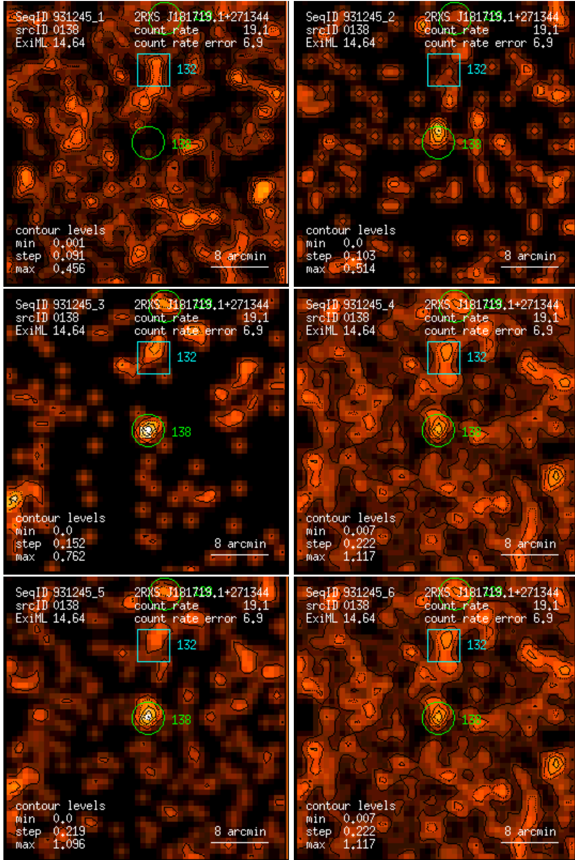
Figure 138: RASS 931245: detection 0138: band rate images, Gaussian filter: (1) PSPC channels 11 – 41, (2) 52 – 90, (3) 91 – 201, (4) 11 – 235, (5) 52 – 201, (6) 11 – 201. Broad band rates in counts/ks. Band rate contour levels in counts/ks/arcmin 2 .
