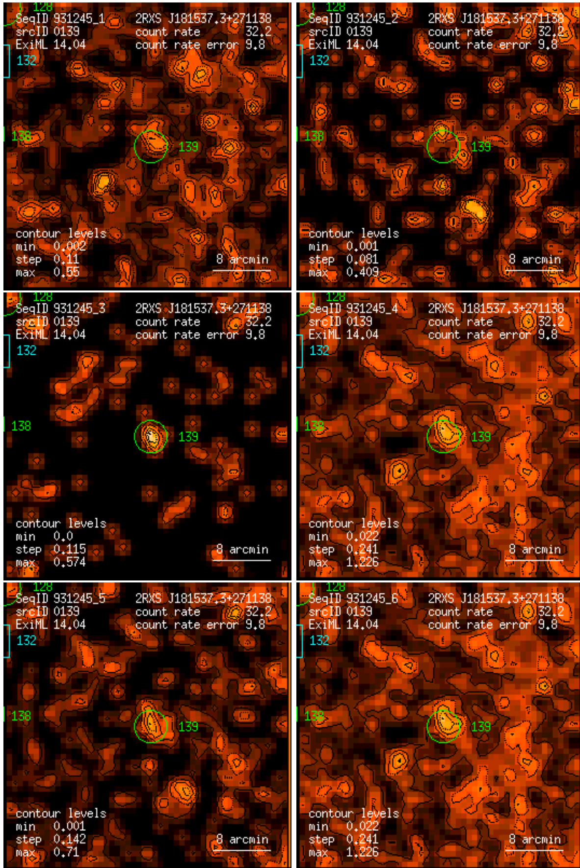
Figure 139: RASS 931245: detection 0139: band rate images, Gaussian filter: (1) PSPC channels 11 – 41, (2) 52 – 90, (3) 91 – 201, (4) 11 – 235, (5) 52 – 201, (6) 11 – 201. Broad band rates in counts/ks. Band rate contour levels in counts/ks/arcmin 2 .
