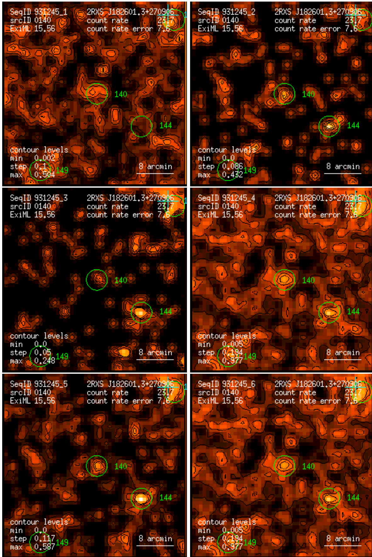
Figure 140: RASS 931245: detection 0140: band rate images, Gaussian filter: (1) PSPC channels 11 – 41, (2) 52 – 90, (3) 91 – 201, (4) 11 – 235, (5) 52 – 201, (6) 11 – 201. Broad band rates in counts/ks. Band rate contour levels in counts/ks/arcmin 2 .
