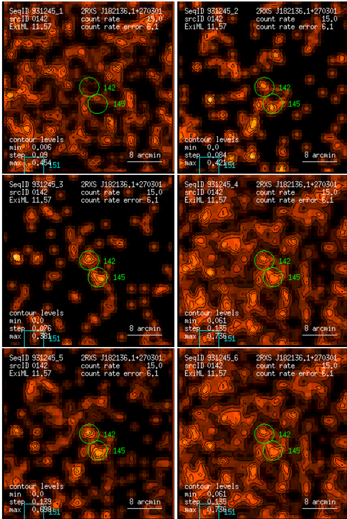
Figure 142: RASS 931245: detection 0142: band rate images, Gaussian filter: (1) PSPC channels 11 – 41, (2) 52 – 90, (3) 91 – 201, (4) 11 – 235, (5) 52 – 201, (6) 11 – 201. Broad band rates in counts/ks. Band rate contour levels in counts/ks/arcmin 2 .
