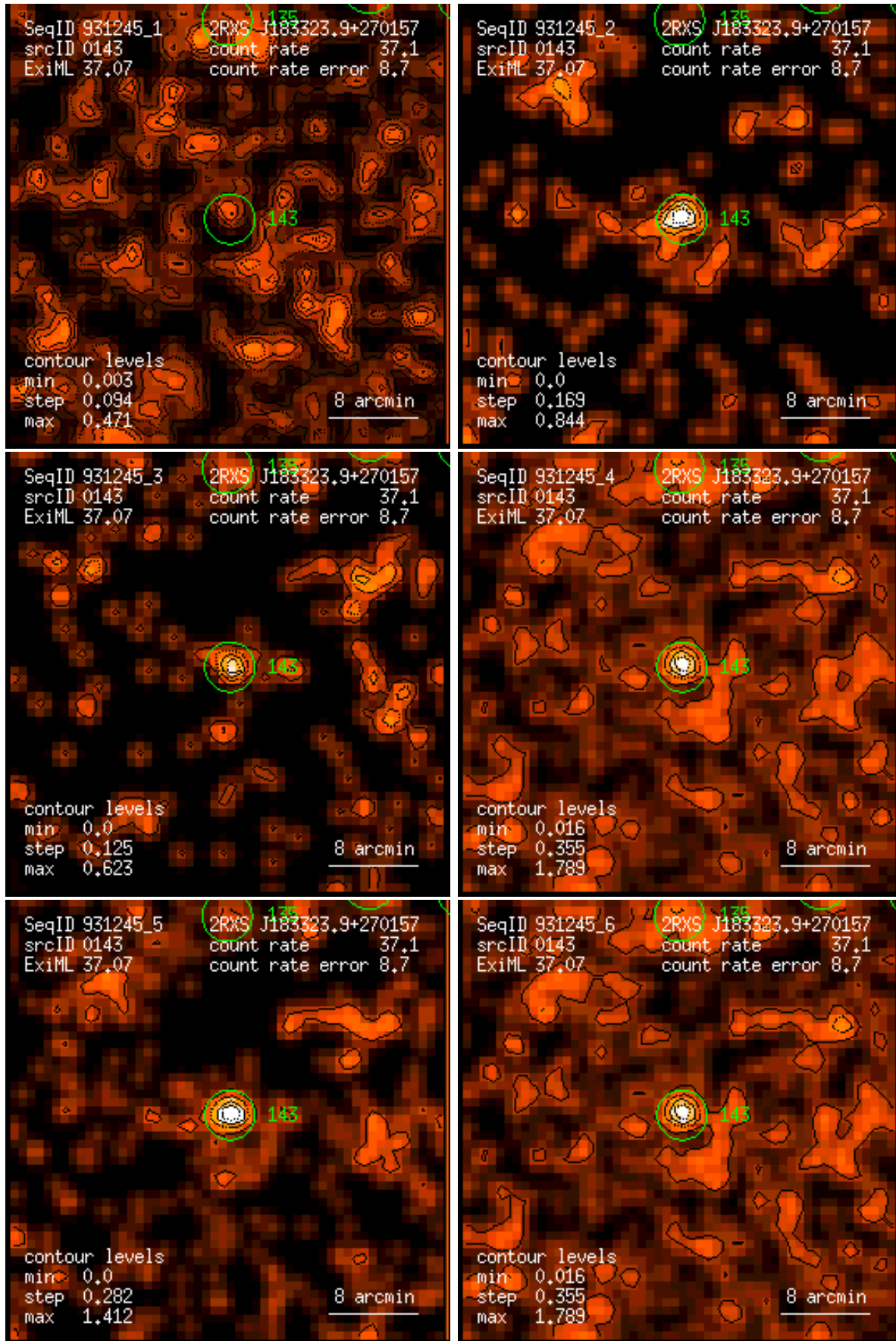
Figure 143: RASS 931245: detection 0143: band rate images, Gaussian filter: (1) PSPC channels 11 – 41, (2) 52 – 90, (3) 91 – 201, (4) 11 – 235, (5) 52 – 201, (6) 11 – 201. Broad band rates in counts/ks. Band rate contour levels in counts/ks/arcmin 2 .
