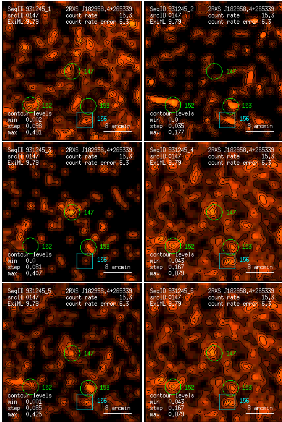
Figure 147: RASS 931245: detection 0147: band rate images, Gaussian filter: (1) PSPC channels 11 – 41, (2) 52 – 90, (3) 91 – 201, (4) 11 – 235, (5) 52 – 201, (6) 11 – 201. Broad band rates in counts/ks. Band rate contour levels in counts/ks/arcmin 2 .
