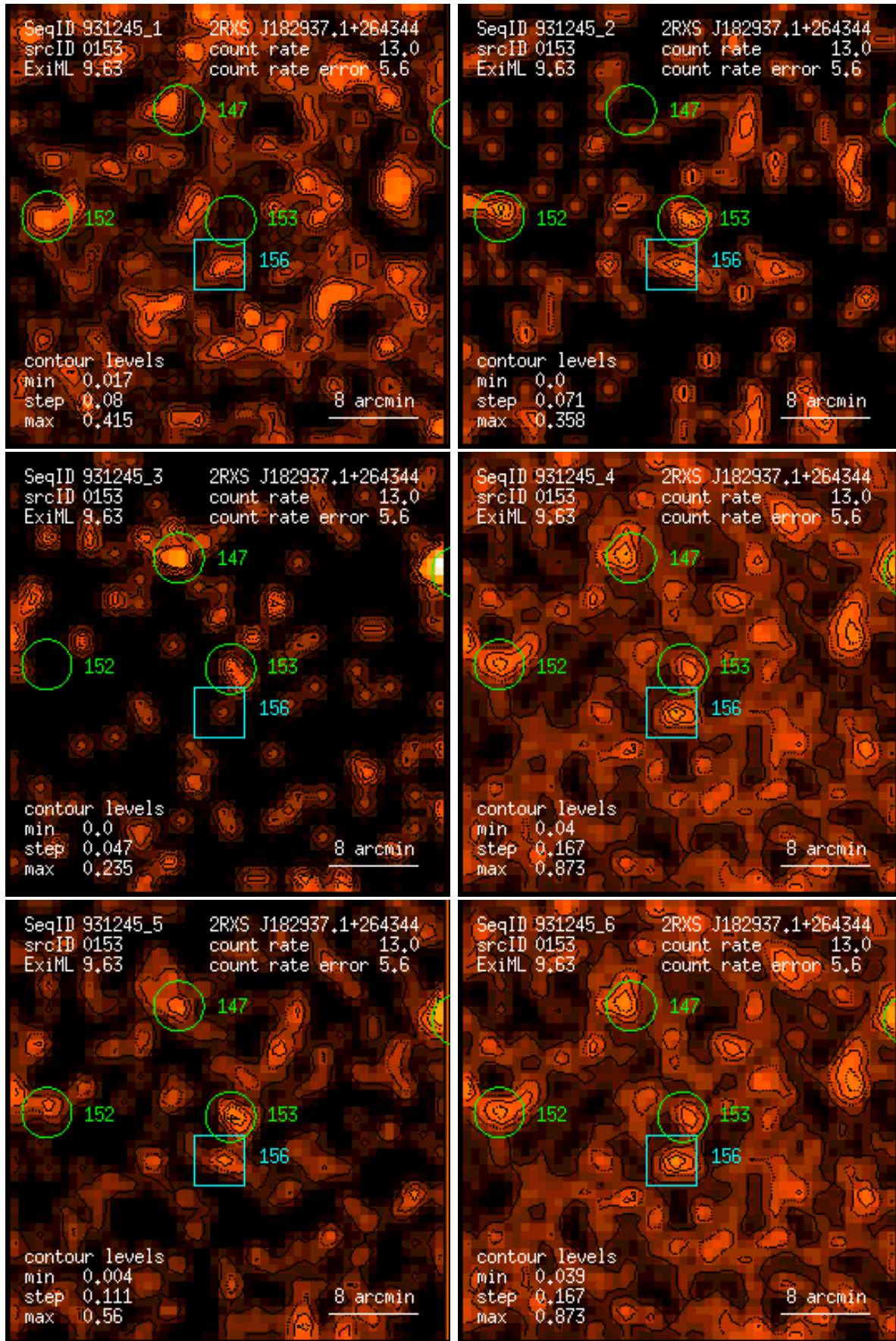
Figure 153: RASS 931245: detection 0153: band rate images, Gaussian filter: (1) PSPC channels 11 – 41, (2) 52 – 90, (3) 91 – 201, (4) 11 – 235, (5) 52 – 201, (6) 11 – 201. Broad band rates in counts/ks. Band rate contour levels in counts/ks/arcmin 2 .
