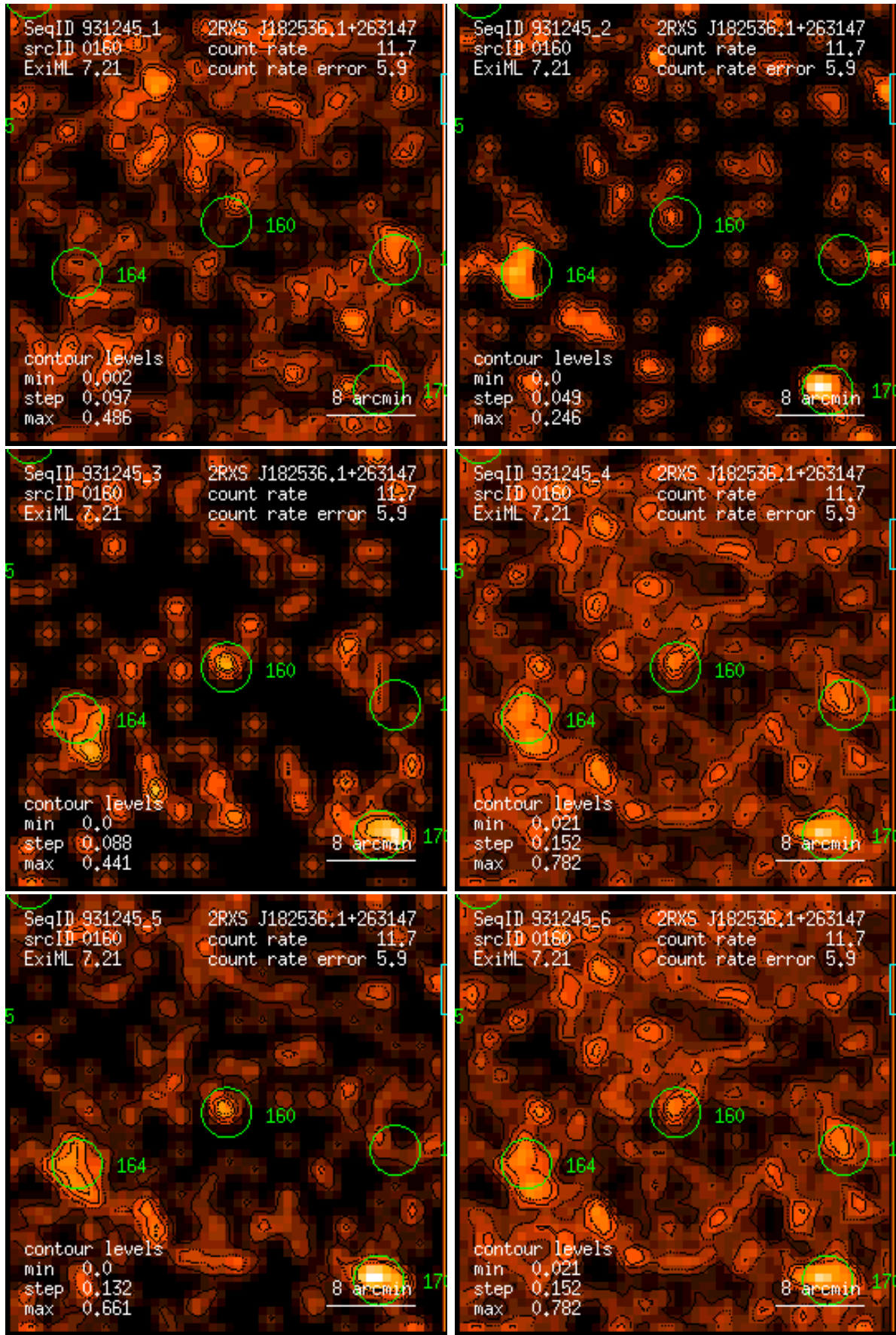
Figure 160: RASS 931245: detection 0160: band rate images, Gaussian filter: (1) PSPC channels 11 – 41, (2) 52 – 90, (3) 91 – 201, (4) 11 – 235, (5) 52 – 201, (6) 11 – 201. Broad band rates in counts/ks. Band rate contour levels in counts/ks/arcmin 2 .
