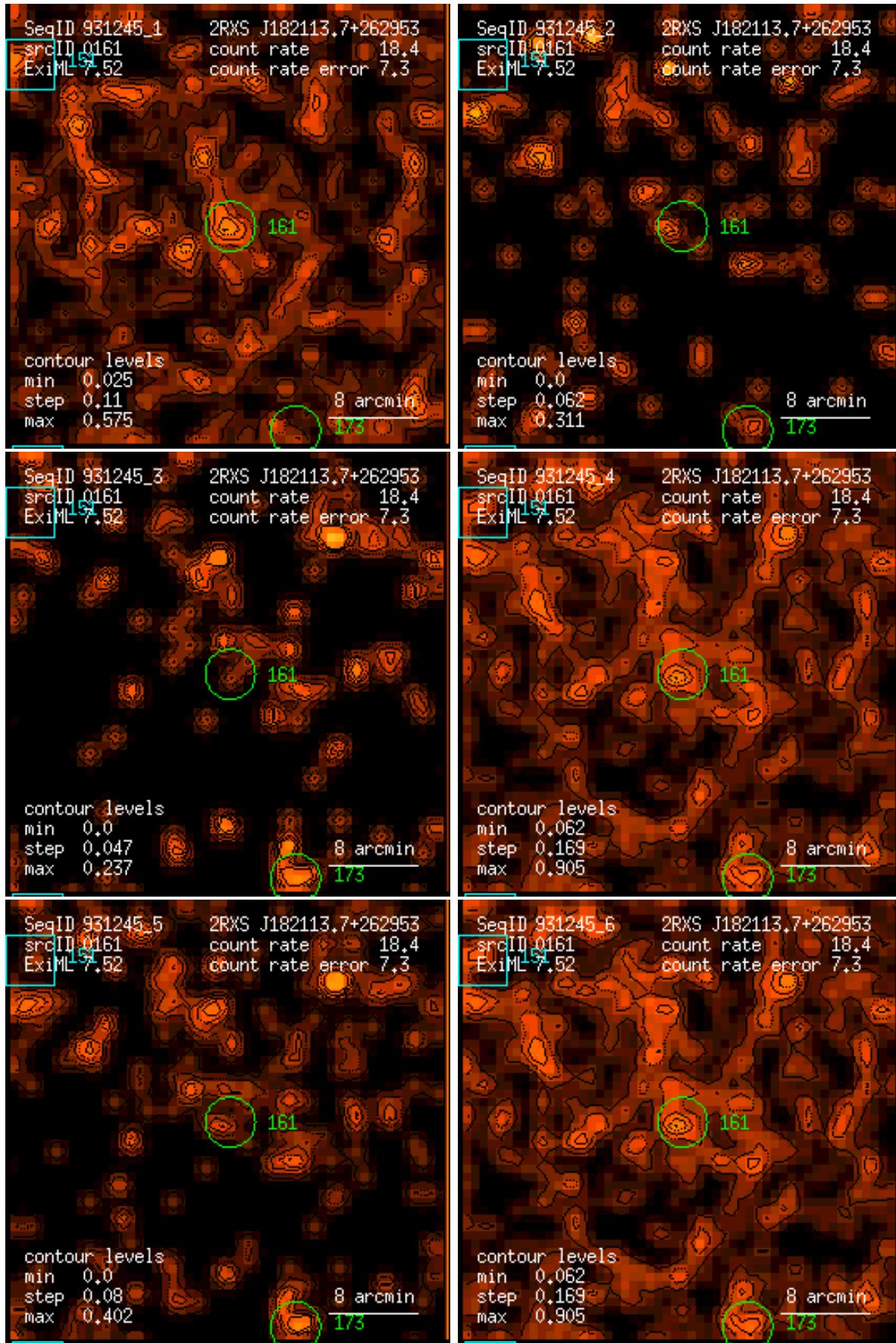
Figure 161: RASS 931245: detection 0161: band rate images, Gaussian filter: (1) PSPC channels 11 – 41, (2) 52 – 90, (3) 91 – 201, (4) 11 – 235, (5) 52 – 201, (6) 11 – 201. Broad band rates in counts/ks. Band rate contour levels in counts/ks/arcmin 2 .
