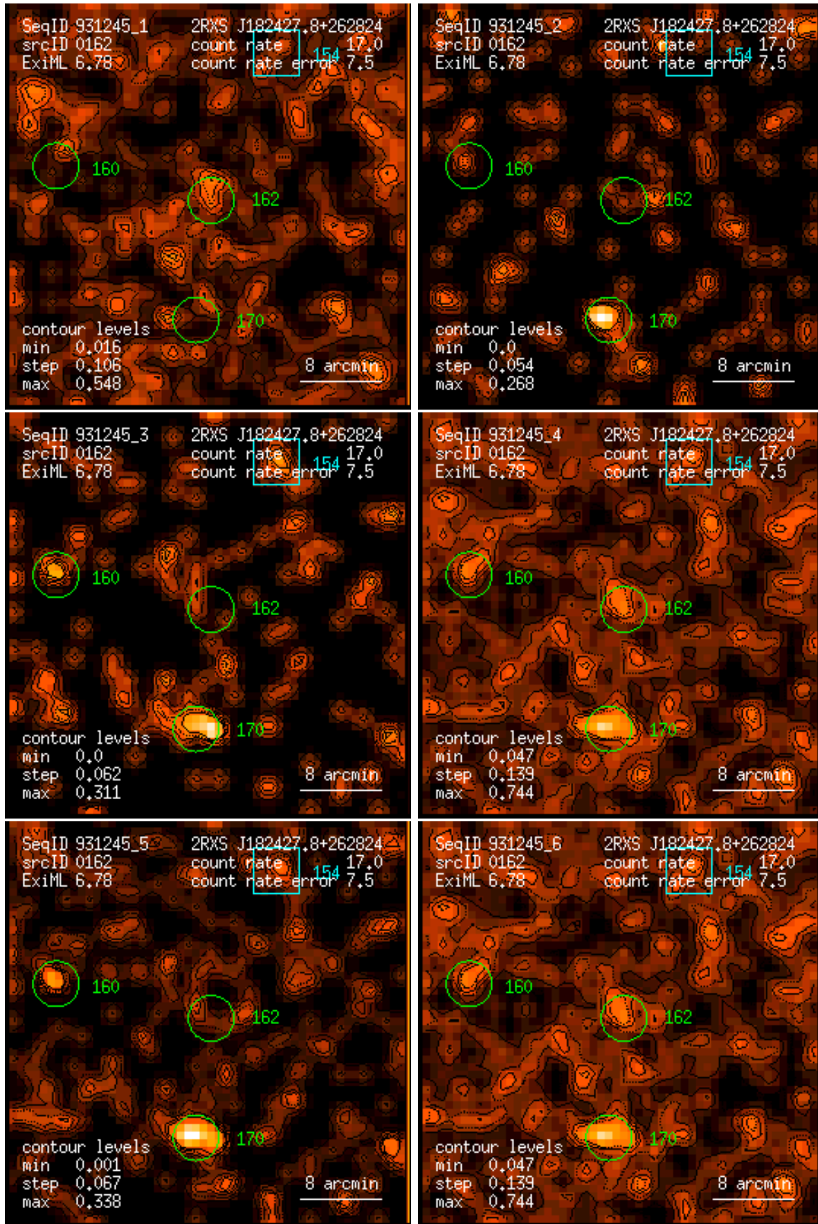
Figure 162: RASS 931245: detection 0162: band rate images, Gaussian filter: (1) PSPC channels 11 – 41, (2) 52 – 90, (3) 91 – 201, (4) 11 – 235, (5) 52 – 201, (6) 11 – 201. Broad band rates in counts/ks. Band rate contour levels in counts/ks/arcmin 2 .
