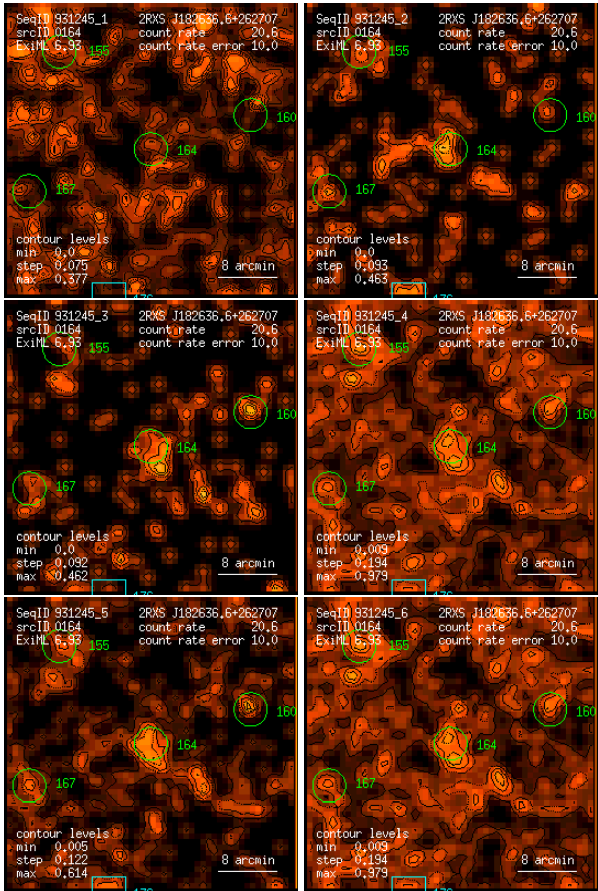
Figure 164: RASS 931245: detection 0164: band rate images, Gaussian filter: (1) PSPC channels 11 – 41, (2) 52 – 90, (3) 91 – 201, (4) 11 – 235, (5) 52 – 201, (6) 11 – 201. Broad band rates in counts/ks. Band rate contour levels in counts/ks/arcmin 2 .
