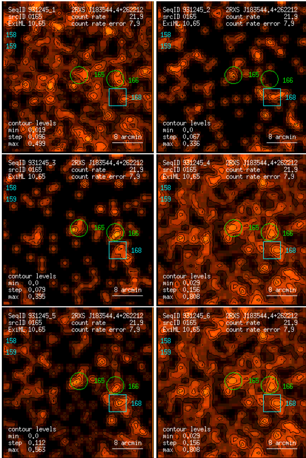
Figure 165: RASS 931245: detection 0165: band rate images, Gaussian filter: (1) PSPC channels 11 – 41, (2) 52 – 90, (3) 91 – 201, (4) 11 – 235, (5) 52 – 201, (6) 11 – 201. Broad band rates in counts/ks. Band rate contour levels in counts/ks/arcmin 2 .
