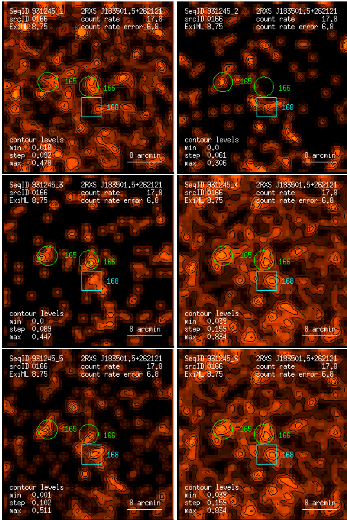
Figure 166: RASS 931245: detection 0166: band rate images, Gaussian filter: (1) PSPC channels 11 – 41, (2) 52 – 90, (3) 91 – 201, (4) 11 – 235, (5) 52 – 201, (6) 11 – 201. Broad band rates in counts/ks. Band rate contour levels in counts/ks/arcmin 2 .
