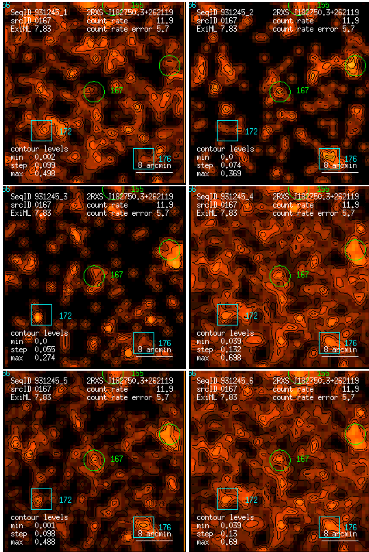
Figure 167: RASS 931245: detection 0167: band rate images, Gaussian filter: (1) PSPC channels 11 – 41, (2) 52 – 90, (3) 91 – 201, (4) 11 – 235, (5) 52 – 201, (6) 11 – 201. Broad band rates in counts/ks. Band rate contour levels in counts/ks/arcmin 2 .
