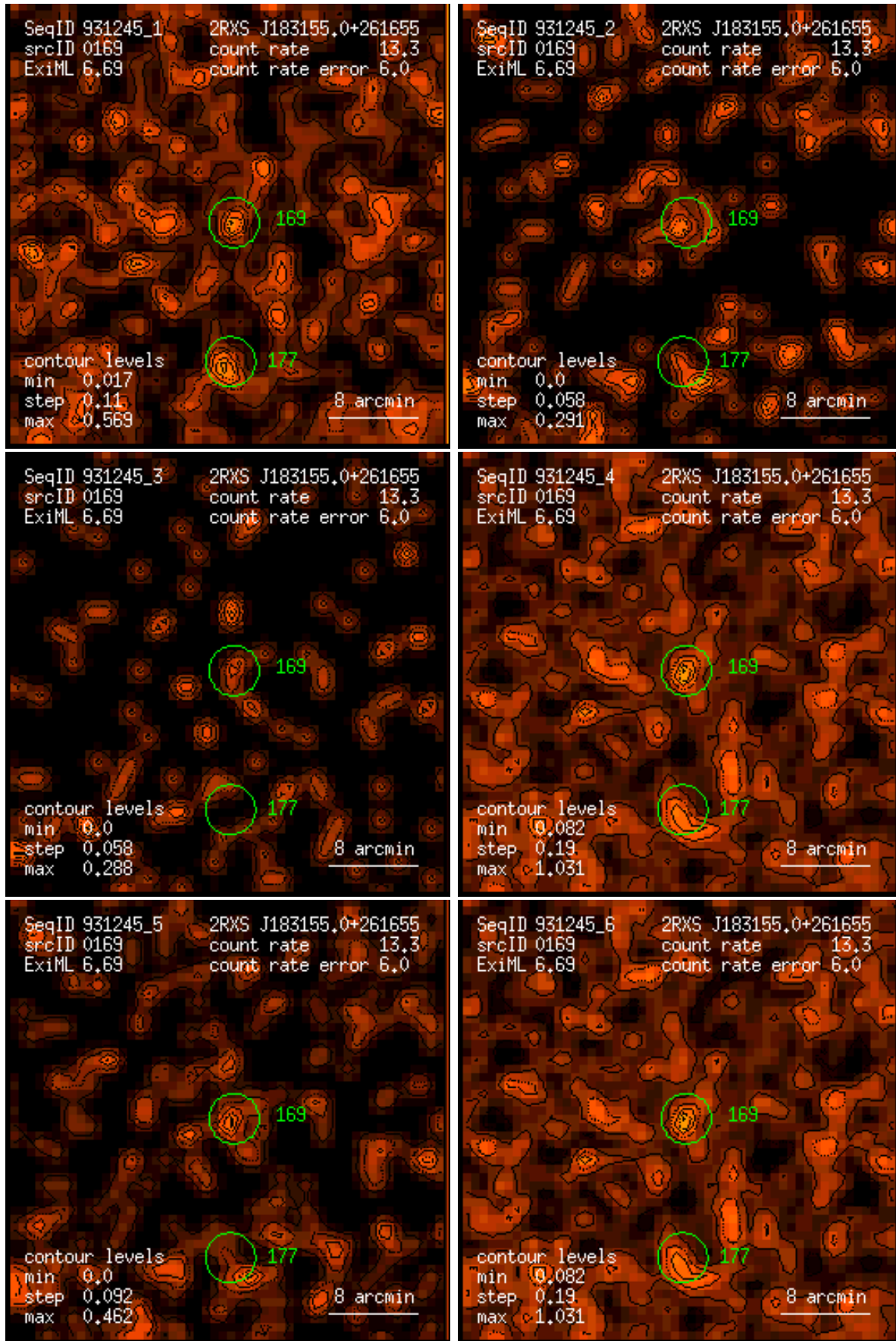
Figure 169: RASS 931245: detection 0169: band rate images, Gaussian filter: (1) PSPC channels 11 – 41, (2) 52 – 90, (3) 91 – 201, (4) 11 – 235, (5) 52 – 201, (6) 11 – 201. Broad band rates in counts/ks. Band rate contour levels in counts/ks/arcmin 2 .
