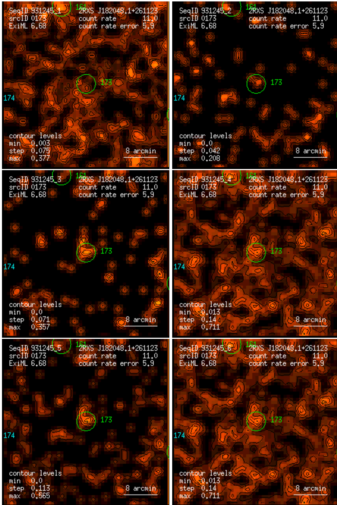
Figure 173: RASS 931245: detection 0173: band rate images, Gaussian filter: (1) PSPC channels 11 – 41, (2) 52 – 90, (3) 91 – 201, (4) 11 – 235, (5) 52 – 201, (6) 11 – 201. Broad band rates in counts/ks. Band rate contour levels in counts/ks/arcmin 2 .
