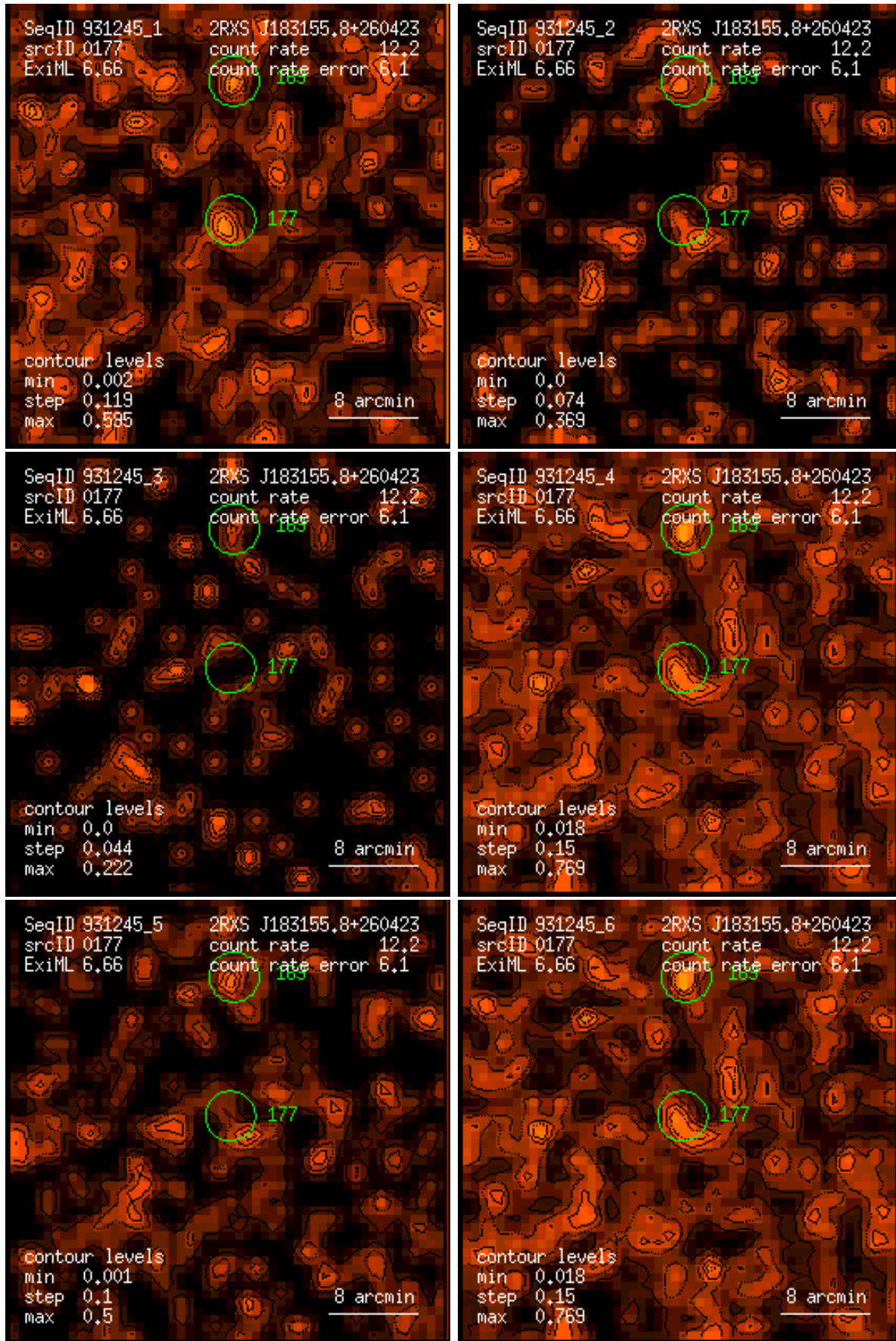
Figure 177: RASS 931245: detection 0177: band rate images, Gaussian filter: (1) PSPC channels 11 – 41, (2) 52 – 90, (3) 91 – 201, (4) 11 – 235, (5) 52 – 201, (6) 11 – 201. Broad band rates in counts/ks. Band rate contour levels in counts/ks/arcmin 2 .
