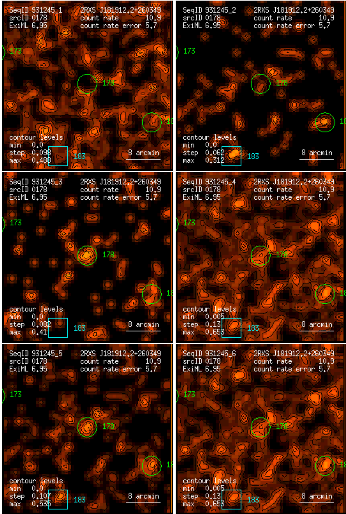
Figure 178: RASS 931245: detection 0178: band rate images, Gaussian filter: (1) PSPC channels 11 – 41, (2) 52 – 90, (3) 91 – 201, (4) 11 – 235, (5) 52 – 201, (6) 11 – 201. Broad band rates in counts/ks. Band rate contour levels in counts/ks/arcmin 2 .
