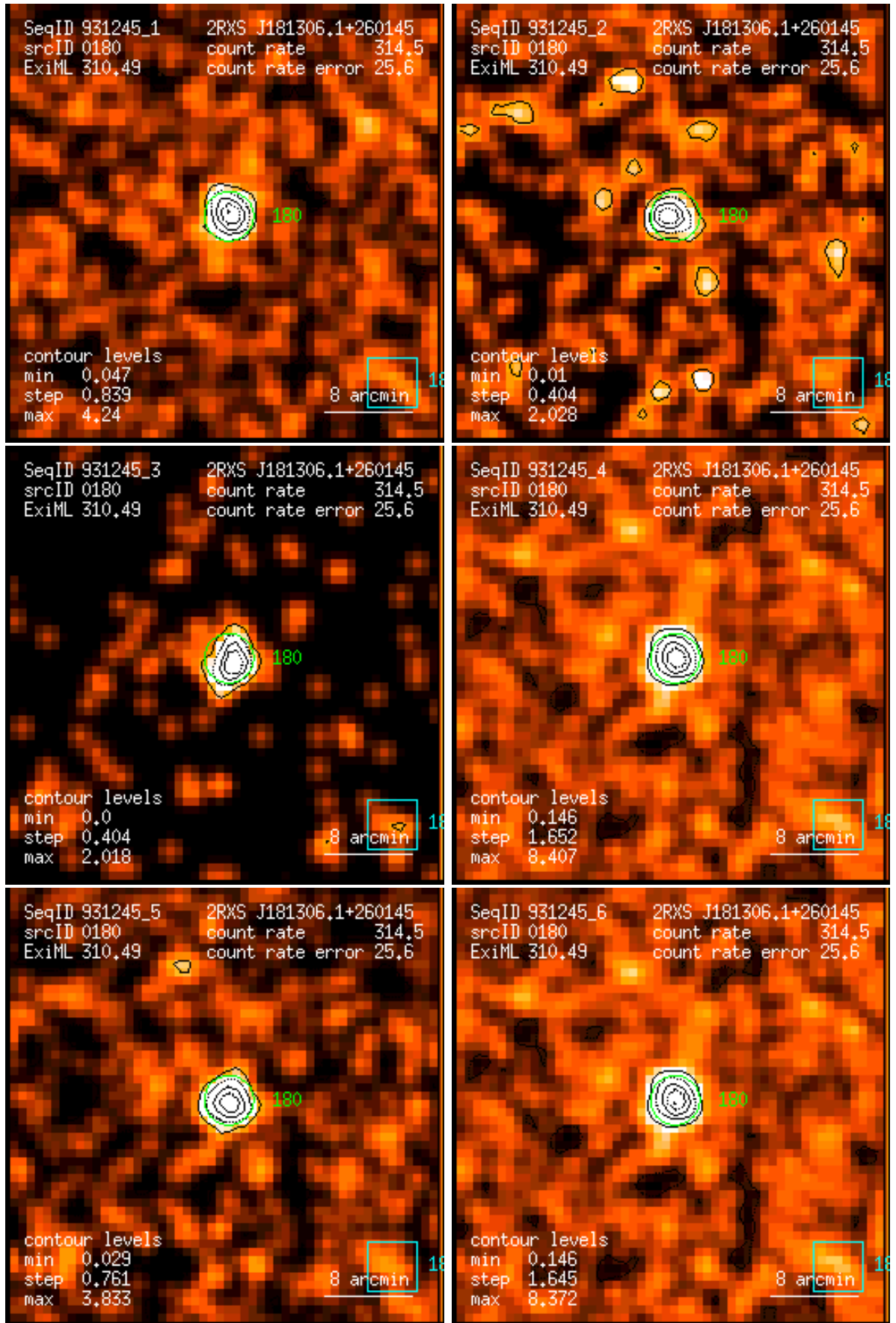
Figure 180: RASS 931245: detection 0180: band rate images, Gaussian filter: (1) PSPC channels 11 – 41, (2) 52 – 90, (3) 91 – 201, (4) 11 – 235, (5) 52 – 201, (6) 11 – 201. Broad band rates in counts/ks. Band rate contour levels in counts/ks/arcmin 2 .
