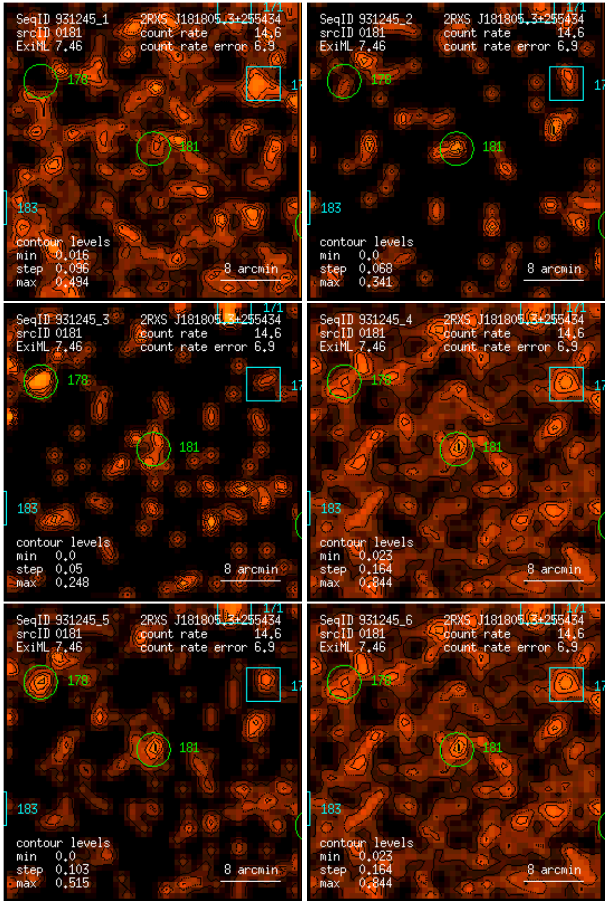
Figure 181: RASS 931245: detection 0181: band rate images, Gaussian filter: (1) PSPC channels 11 – 41, (2) 52 – 90, (3) 91 – 201, (4) 11 – 235, (5) 52 – 201, (6) 11 – 201. Broad band rates in counts/ks. Band rate contour levels in counts/ks/arcmin 2 .
