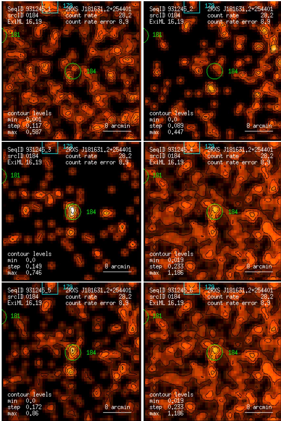
Figure 184: RASS 931245: detection 0184: band rate images, Gaussian filter: (1) PSPC channels 11 – 41, (2) 52 – 90, (3) 91 – 201, (4) 11 – 235, (5) 52 – 201, (6) 11 – 201. Broad band rates in counts/ks. Band rate contour levels in counts/ks/arcmin 2 .
