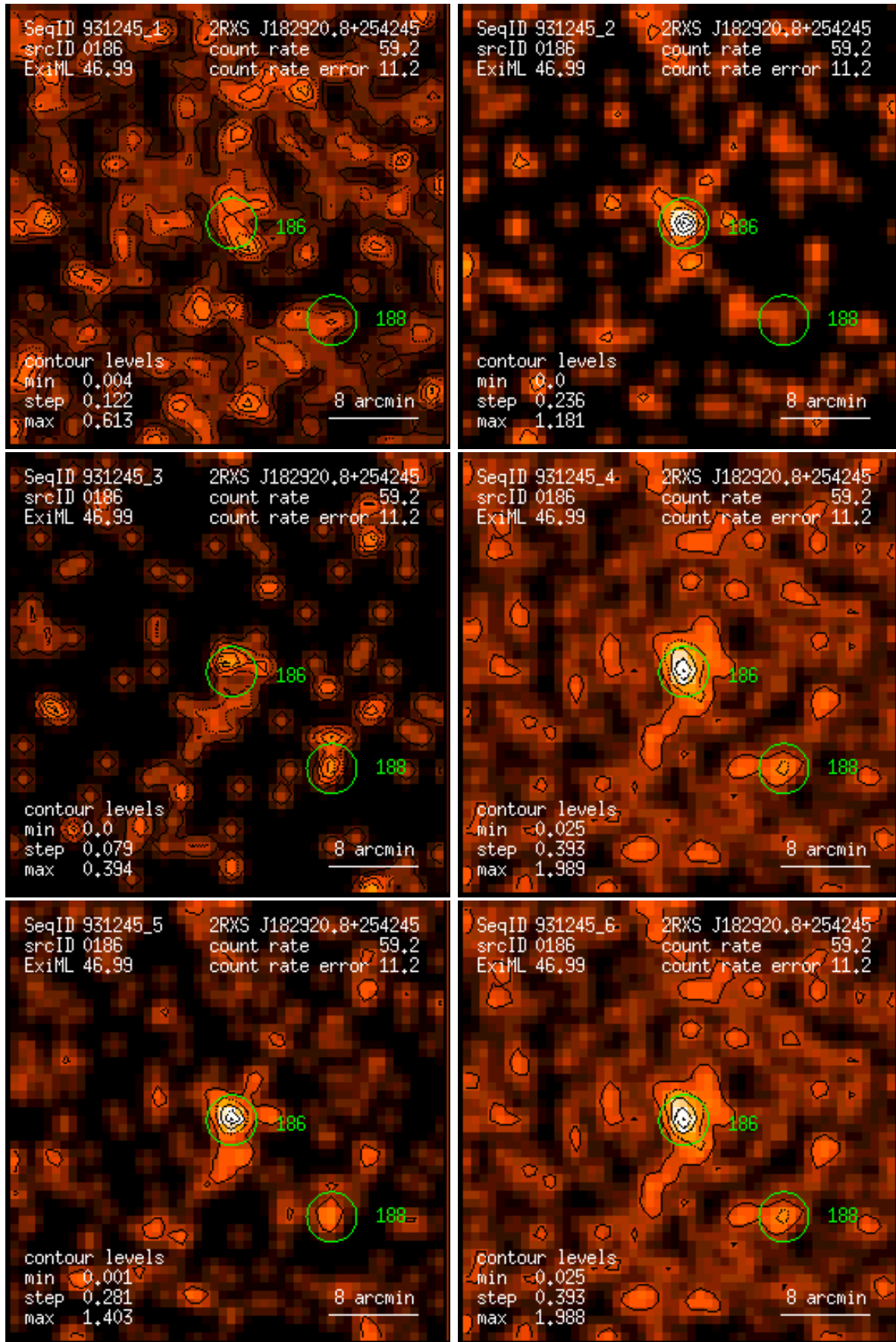
Figure 186: RASS 931245: detection 0186: band rate images, Gaussian filter: (1) PSPC channels 11 – 41, (2) 52 – 90, (3) 91 – 201, (4) 11 – 235, (5) 52 – 201, (6) 11 – 201. Broad band rates in counts/ks. Band rate contour levels in counts/ks/arcmin 2 .
