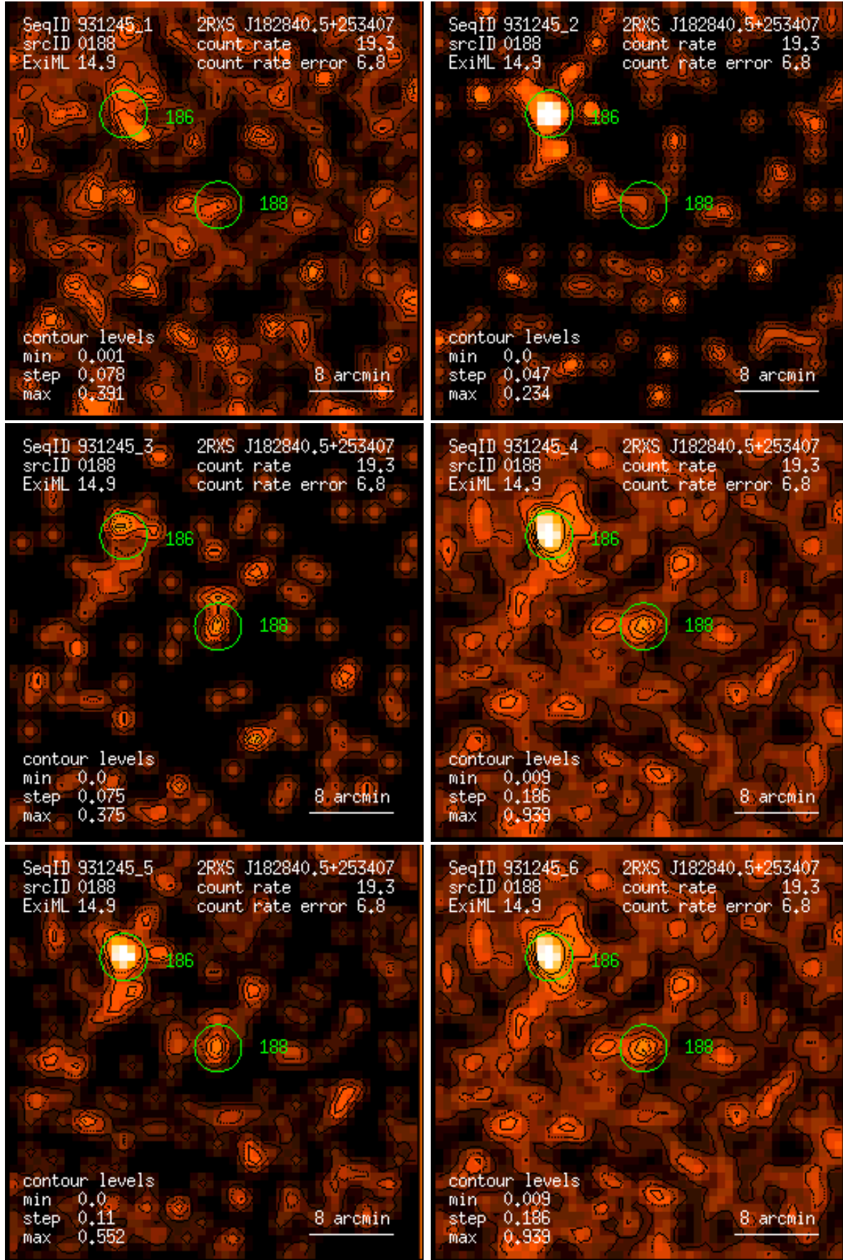
Figure 188: RASS 931245: detection 0188: band rate images, Gaussian filter: (1) PSPC channels 11 – 41, (2) 52 – 90, (3) 91 – 201, (4) 11 – 235, (5) 52 – 201, (6) 11 – 201. Broad band rates in counts/ks. Band rate contour levels in counts/ks/arcmin 2 .
