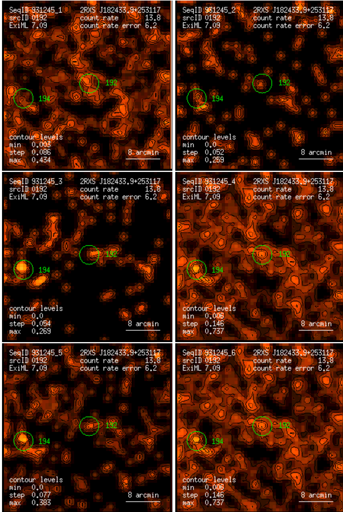
Figure 192: RASS 931245: detection 0192: band rate images, Gaussian filter: (1) PSPC channels 11 – 41, (2) 52 – 90, (3) 91 – 201, (4) 11 – 235, (5) 52 – 201, (6) 11 – 201. Broad band rates in counts/ks. Band rate contour levels in counts/ks/arcmin 2 .
