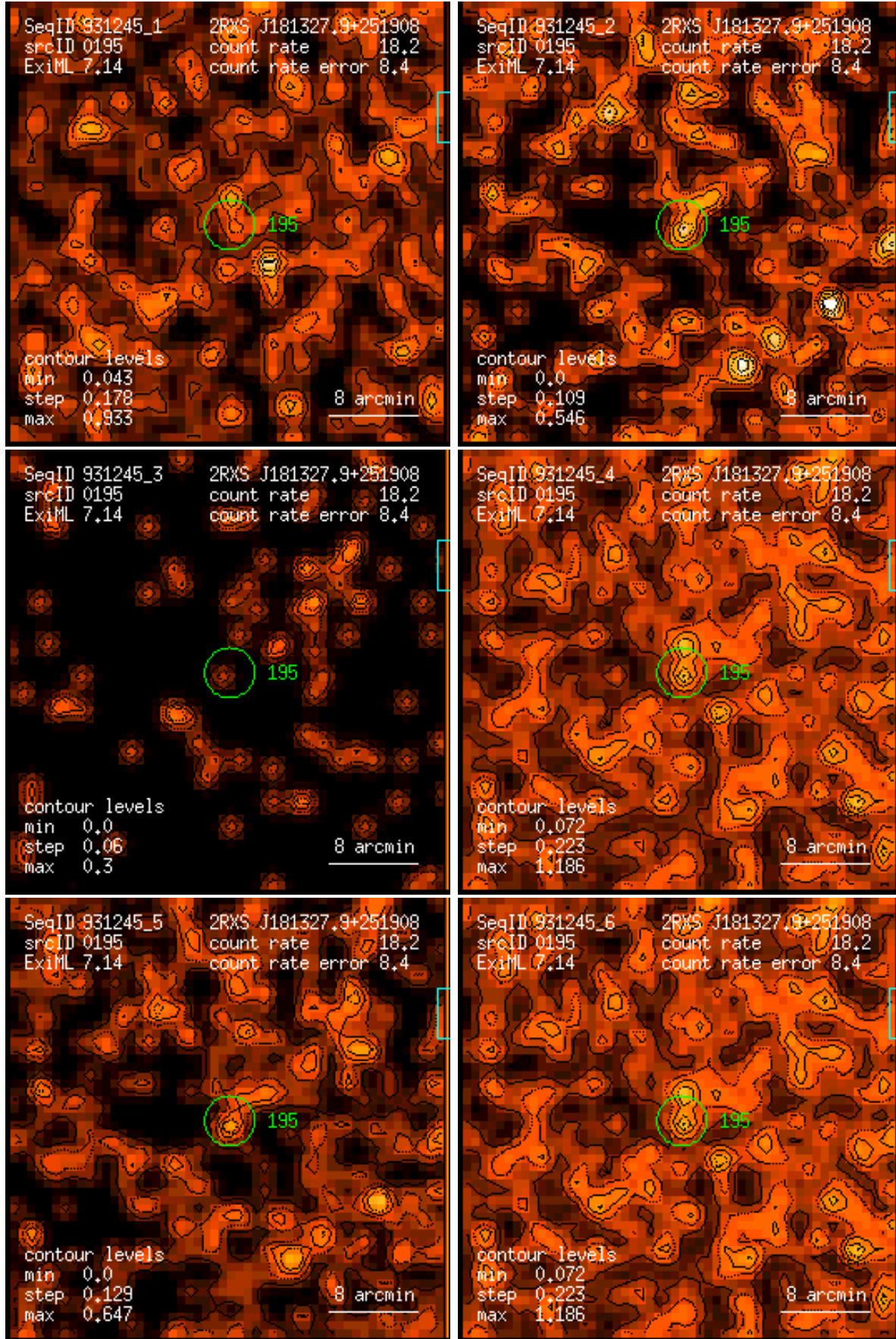
Figure 195: RASS 931245: detection 0195: band rate images, Gaussian filter: (1) PSPC channels 11 – 41, (2) 52 – 90, (3) 91 – 201, (4) 11 – 235, (5) 52 – 201, (6) 11 – 201. Broad band rates in counts/ks. Band rate contour levels in counts/ks/arcmin 2 .
