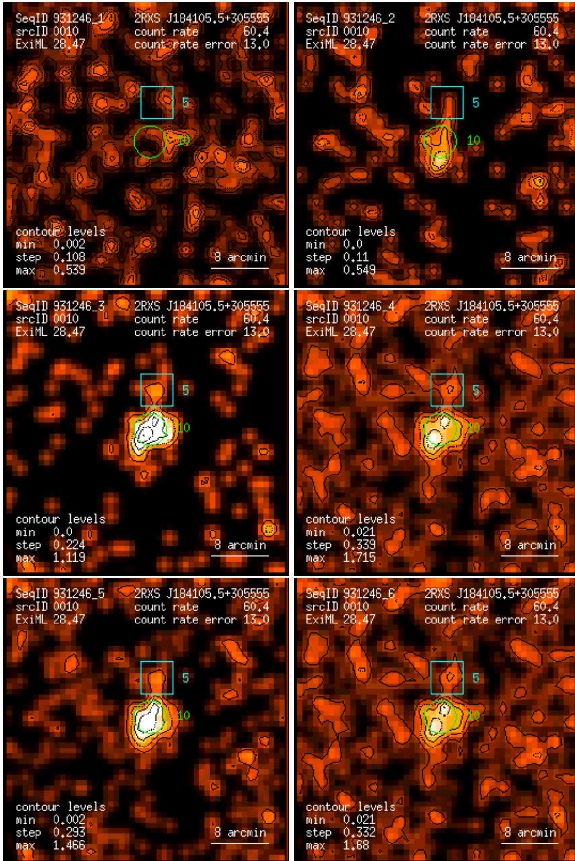
Figure 10: RASS 931246: detection 0010: band rate images, Gaussian filter: (1) PSPC channels 11 – 41, (2) 52 – 90, (3) 91 – 201, (4) 11 – 235, (5) 52 – 201, (6) 11 – 201. Broad band rates in counts/ks. Band rate contour levels in counts/ks/arcmin 2 .
