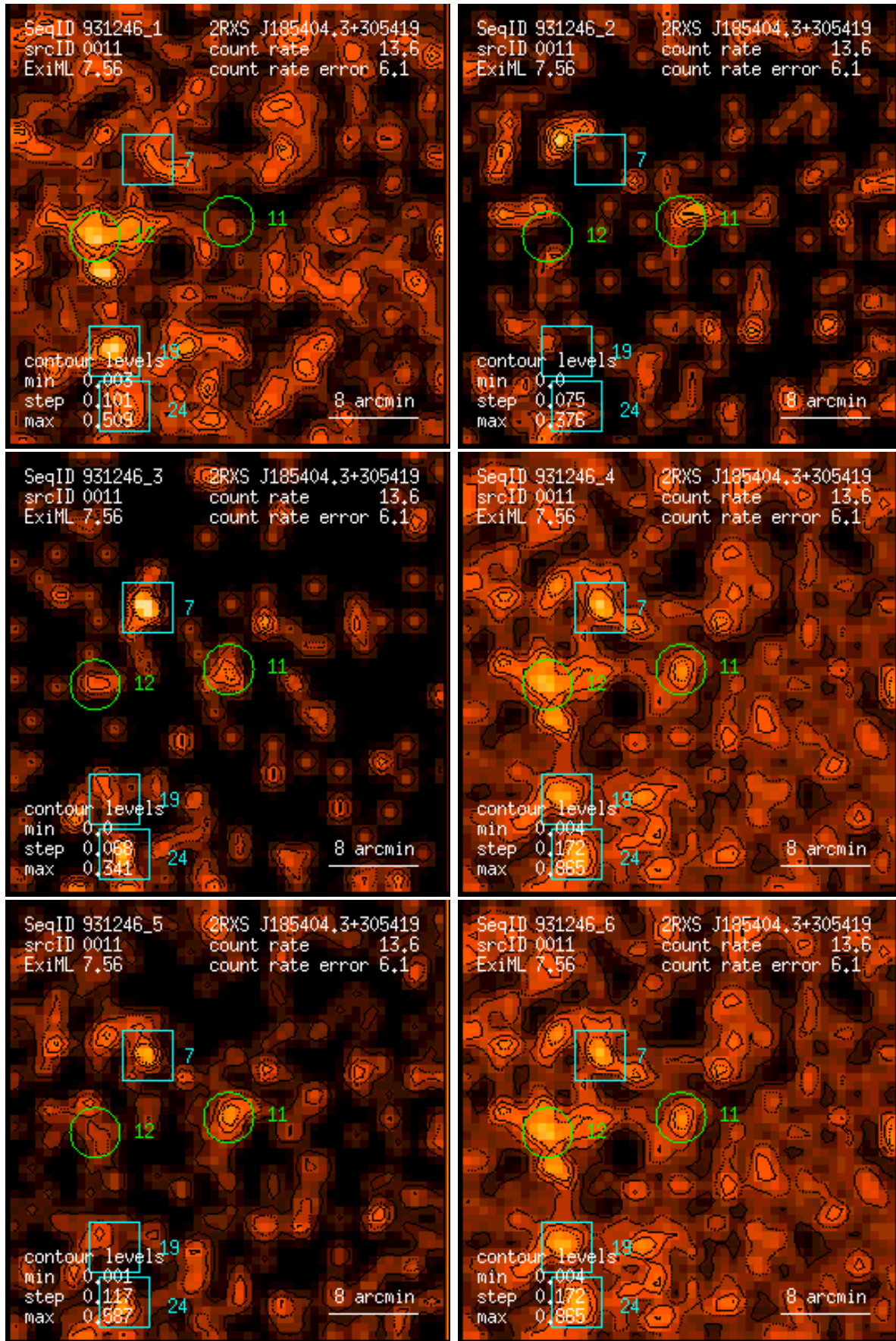
Figure 11: RASS 931246: detection 0011: band rate images, Gaussian filter: (1) PSPC channels 11 – 41, (2) 52 – 90, (3) 91 – 201, (4) 11 – 235, (5) 52 – 201, (6) 11 – 201. Broad band rates in counts/ks. Band rate contour levels in counts/ks/arcmin 2 .
