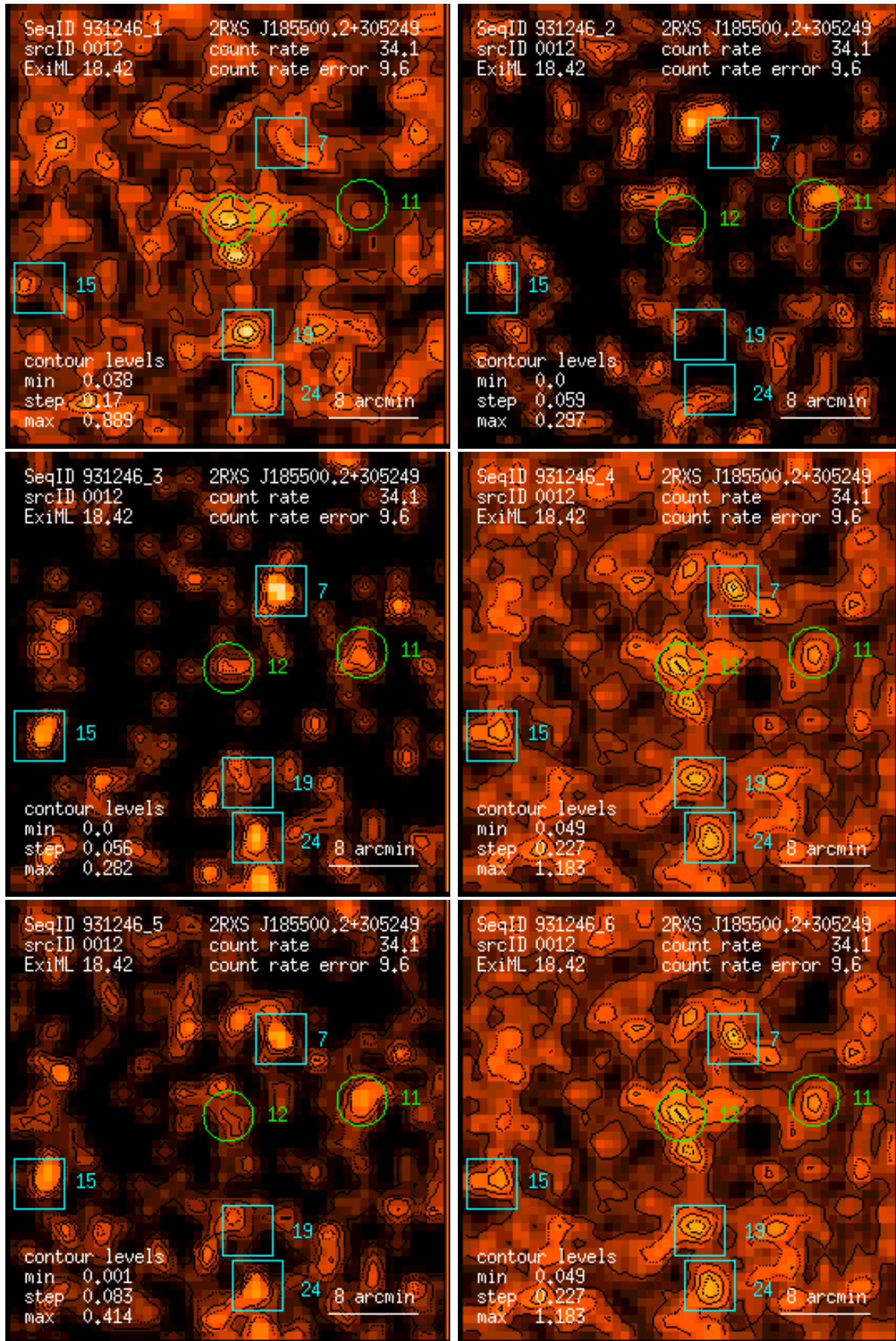
Figure 12: RASS 931246: detection 0012: band rate images, Gaussian filter: (1) PSPC channels 11 – 41, (2) 52 – 90, (3) 91 – 201, (4) 11 – 235, (5) 52 – 201, (6) 11 – 201. Broad band rates in counts/ks. Band rate contour levels in counts/ks/arcmin 2 .
