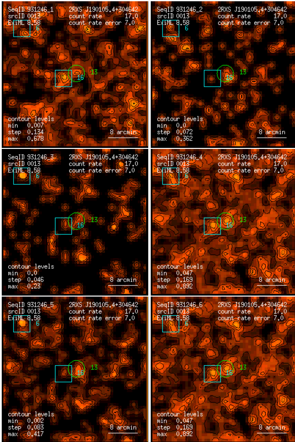
Figure 13: RASS 931246: detection 0013: band rate images, Gaussian filter: (1) PSPC channels 11 – 41, (2) 52 – 90, (3) 91 – 201, (4) 11 – 235, (5) 52 – 201, (6) 11 – 201. Broad band rates in counts/ks. Band rate contour levels in counts/ks/arcmin 2 .
