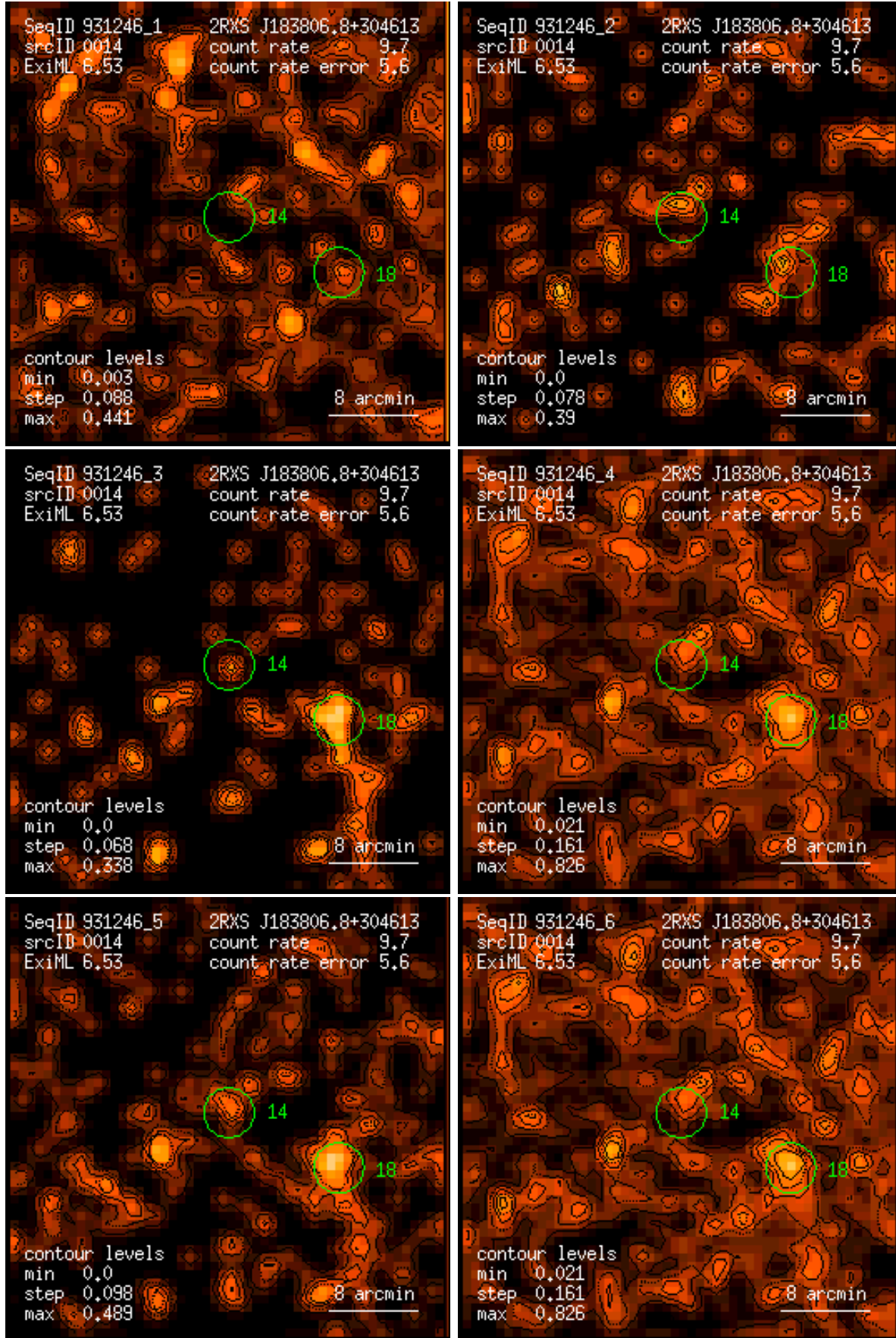
Figure 14: RASS 931246: detection 0014: band rate images, Gaussian filter: (1) PSPC channels 11 – 41, (2) 52 – 90, (3) 91 – 201, (4) 11 – 235, (5) 52 – 201, (6) 11 – 201. Broad band rates in counts/ks. Band rate contour levels in counts/ks/arcmin 2 .
