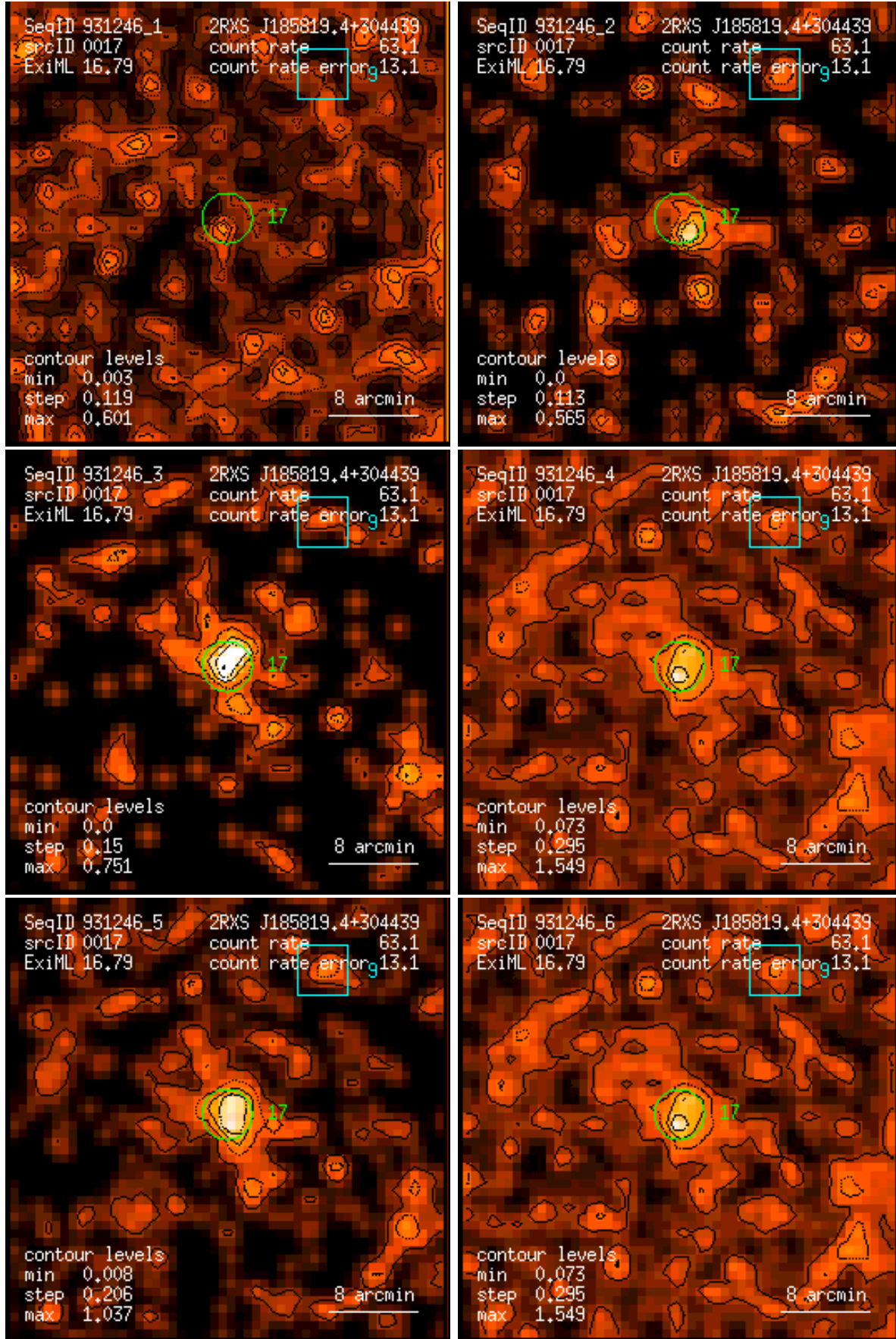
Figure 17: RASS 931246: detection 0017: band rate images, Gaussian filter: (1) PSPC channels 11 – 41, (2) 52 – 90, (3) 91 – 201, (4) 11 – 235, (5) 52 – 201, (6) 11 – 201. Broad band rates in counts/ks. Band rate contour levels in counts/ks/arcmin 2 .
