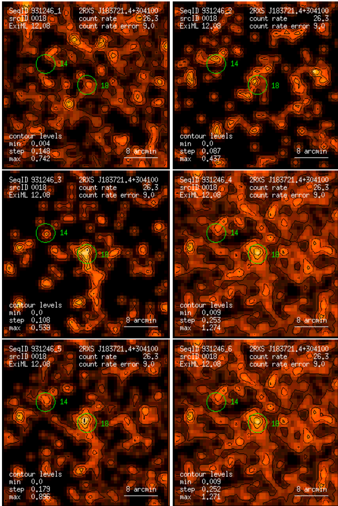
Figure 18: RASS 931246: detection 0018: band rate images, Gaussian filter: (1) PSPC channels 11 – 41, (2) 52 – 90, (3) 91 – 201, (4) 11 – 235, (5) 52 – 201, (6) 11 – 201. Broad band rates in counts/ks. Band rate contour levels in counts/ks/arcmin 2 .
