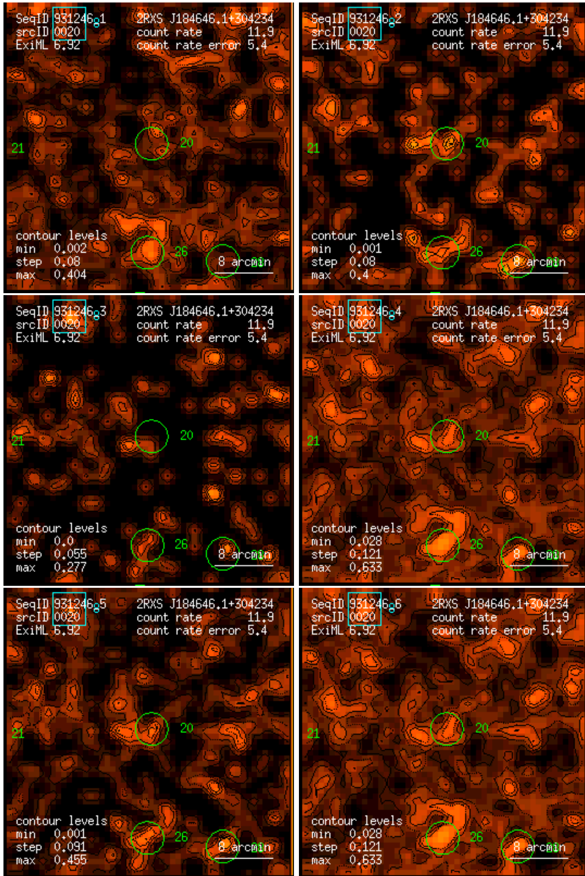
Figure 20: RASS 931246: detection 0020: band rate images, Gaussian filter: (1) PSPC channels 11 – 41, (2) 52 – 90, (3) 91 – 201, (4) 11 – 235, (5) 52 – 201, (6) 11 – 201. Broad band rates in counts/ks. Band rate contour levels in counts/ks/arcmin 2 .
