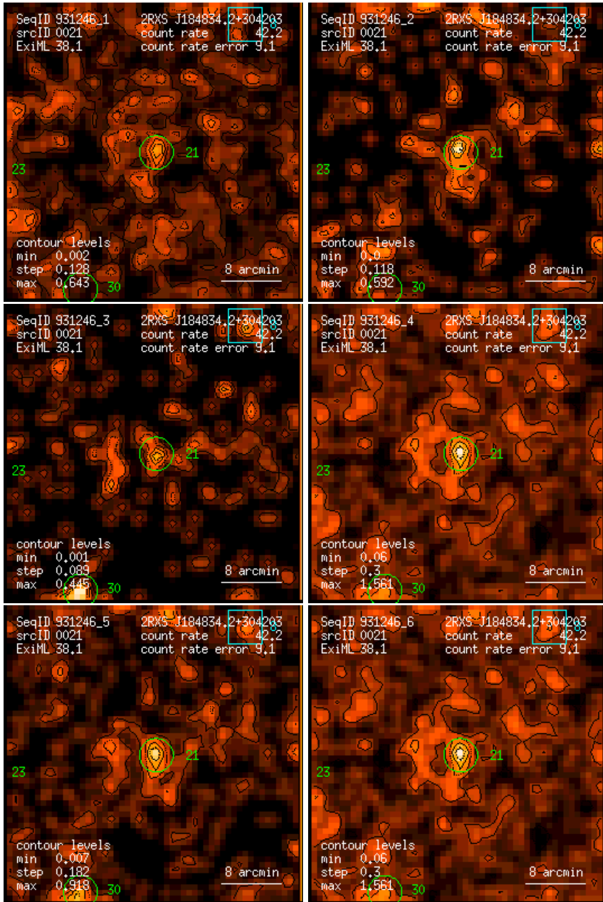
Figure 21: RASS 931246: detection 0021: band rate images, Gaussian filter: (1) PSPC channels 11 – 41, (2) 52 – 90, (3) 91 – 201, (4) 11 – 235, (5) 52 – 201, (6) 11 – 201. Broad band rates in counts/ks. Band rate contour levels in counts/ks/arcmin 2 .
