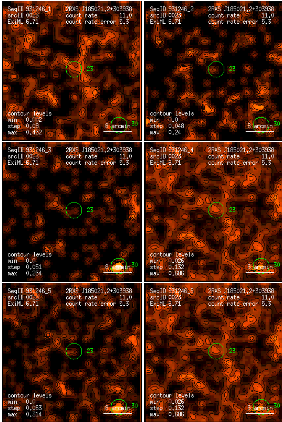
Figure 23: RASS 931246: detection 0023: band rate images, Gaussian filter: (1) PSPC channels 11 – 41, (2) 52 – 90, (3) 91 – 201, (4) 11 – 235, (5) 52 – 201, (6) 11 – 201. Broad band rates in counts/ks. Band rate contour levels in counts/ks/arcmin 2 .
