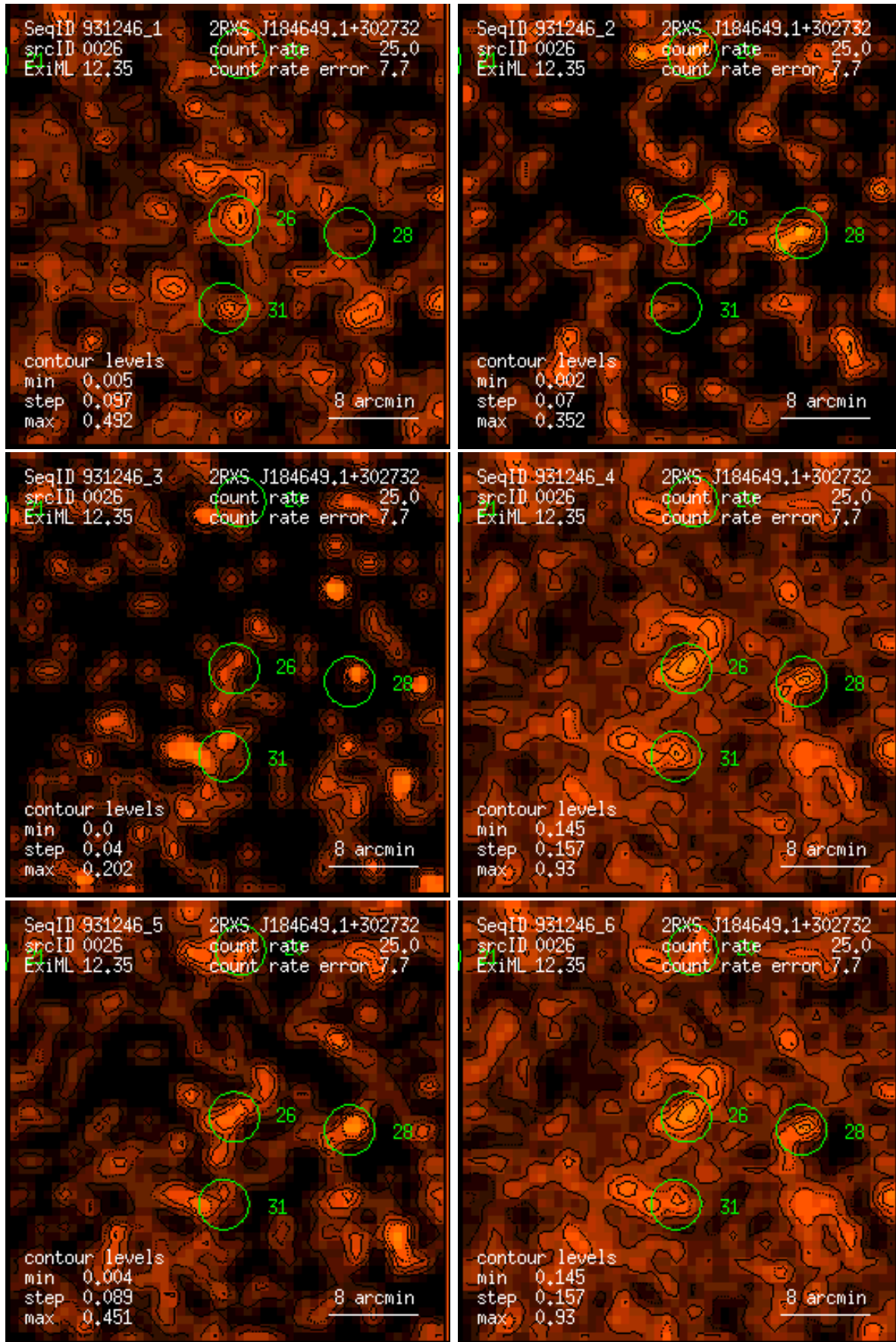
Figure 26: RASS 931246: detection 0026: band rate images, Gaussian filter: (1) PSPC channels 11 – 41, (2) 52 – 90, (3) 91 – 201, (4) 11 – 235, (5) 52 – 201, (6) 11 – 201. Broad band rates in counts/ks. Band rate contour levels in counts/ks/arcmin 2 .
