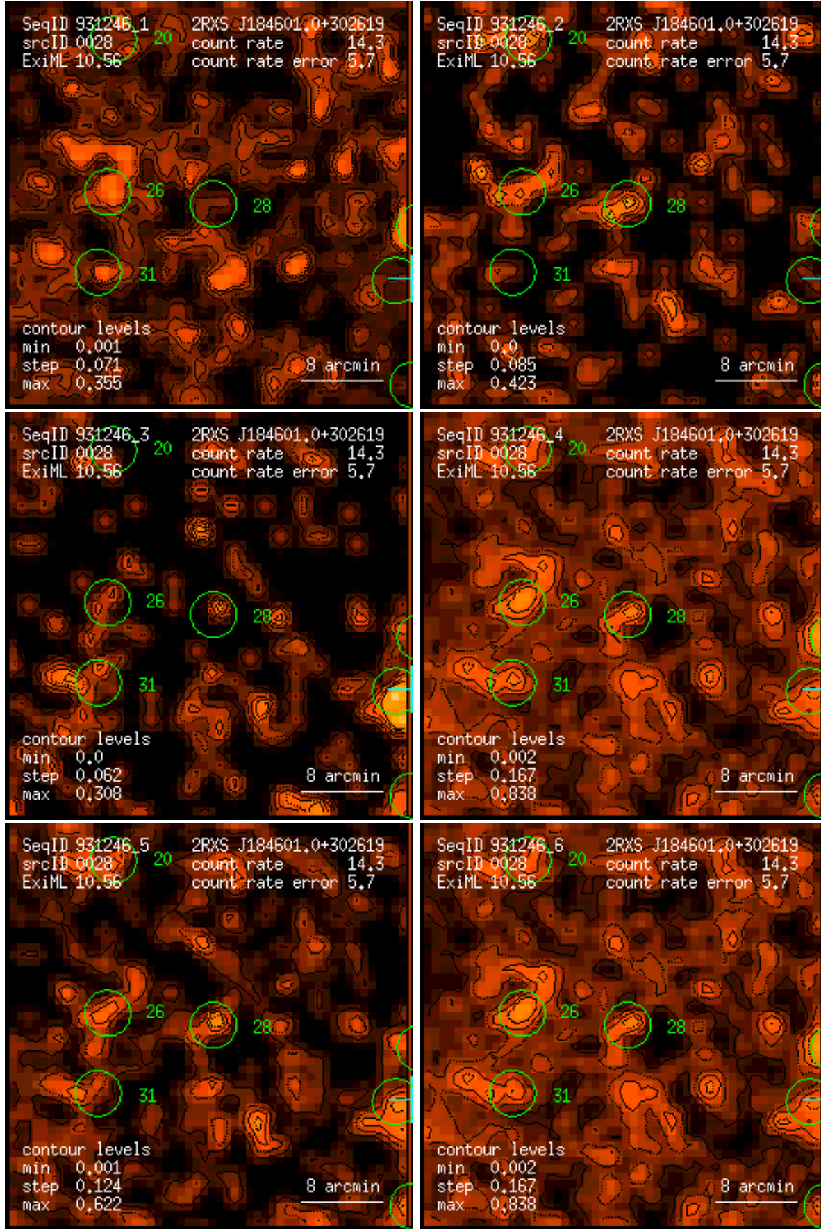
Figure 28: RASS 931246: detection 0028: band rate images, Gaussian filter: (1) PSPC channels 11 – 41, (2) 52 – 90, (3) 91 – 201, (4) 11 – 235, (5) 52 – 201, (6) 11 – 201. Broad band rates in counts/ks. Band rate contour levels in counts/ks/arcmin 2 .
