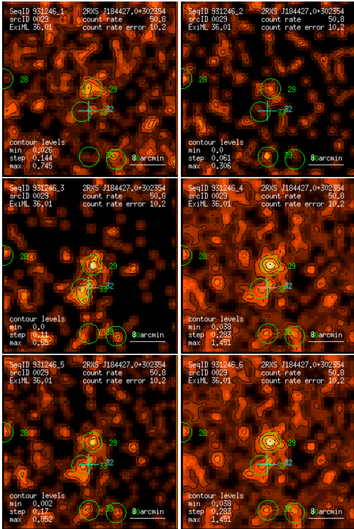
Figure 29: RASS 931246: detection 0029: band rate images, Gaussian filter: (1) PSPC channels 11 – 41, (2) 52 – 90, (3) 91 – 201, (4) 11 – 235, (5) 52 – 201, (6) 11 – 201. Broad band rates in counts/ks. Band rate contour levels in counts/ks/arcmin 2 .
