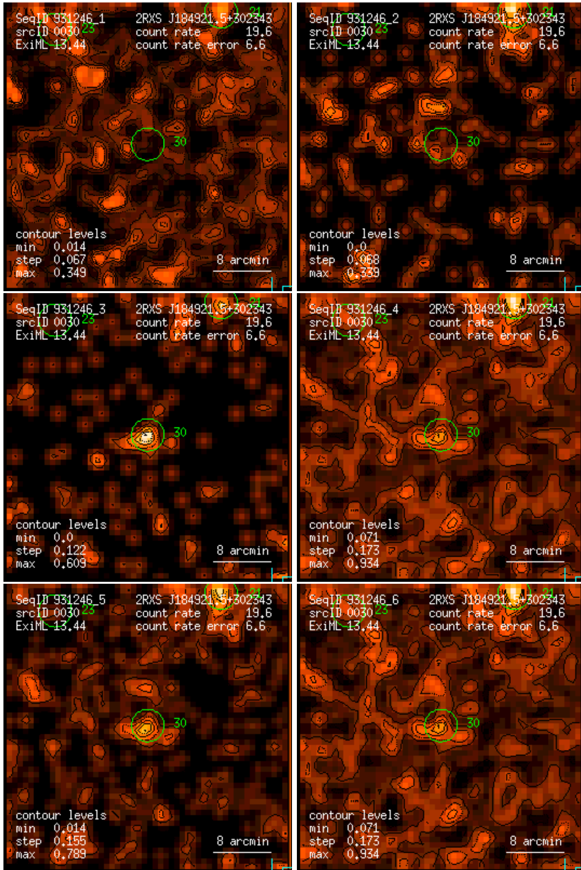
Figure 30: RASS 931246: detection 0030: band rate images, Gaussian filter: (1) PSPC channels 11 – 41, (2) 52 – 90, (3) 91 – 201, (4) 11 – 235, (5) 52 – 201, (6) 11 – 201. Broad band rates in counts/ks. Band rate contour levels in counts/ks/arcmin 2 .
