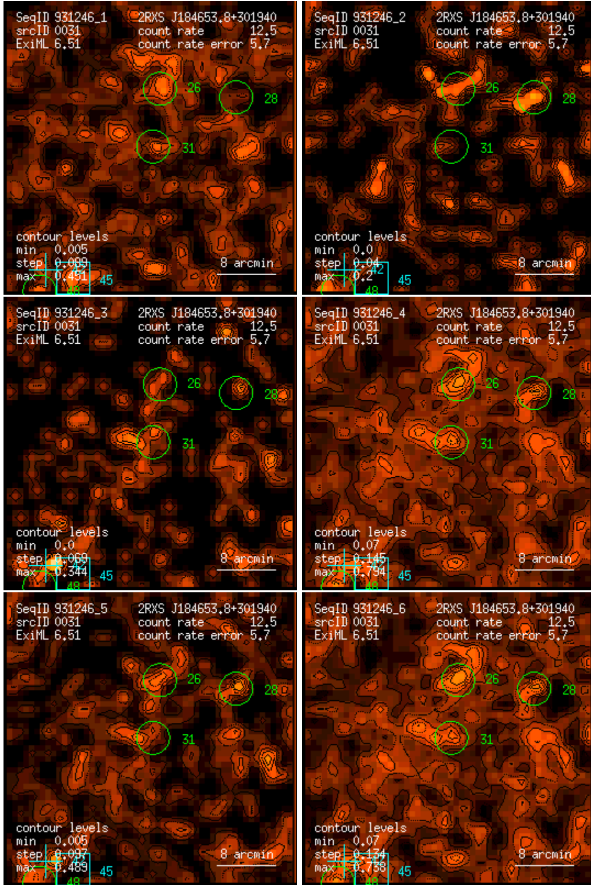
Figure 31: RASS 931246: detection 0031: band rate images, Gaussian filter: (1) PSPC channels 11 – 41, (2) 52 – 90, (3) 91 – 201, (4) 11 – 235, (5) 52 – 201, (6) 11 – 201. Broad band rates in counts/ks. Band rate contour levels in counts/ks/arcmin 2 .
