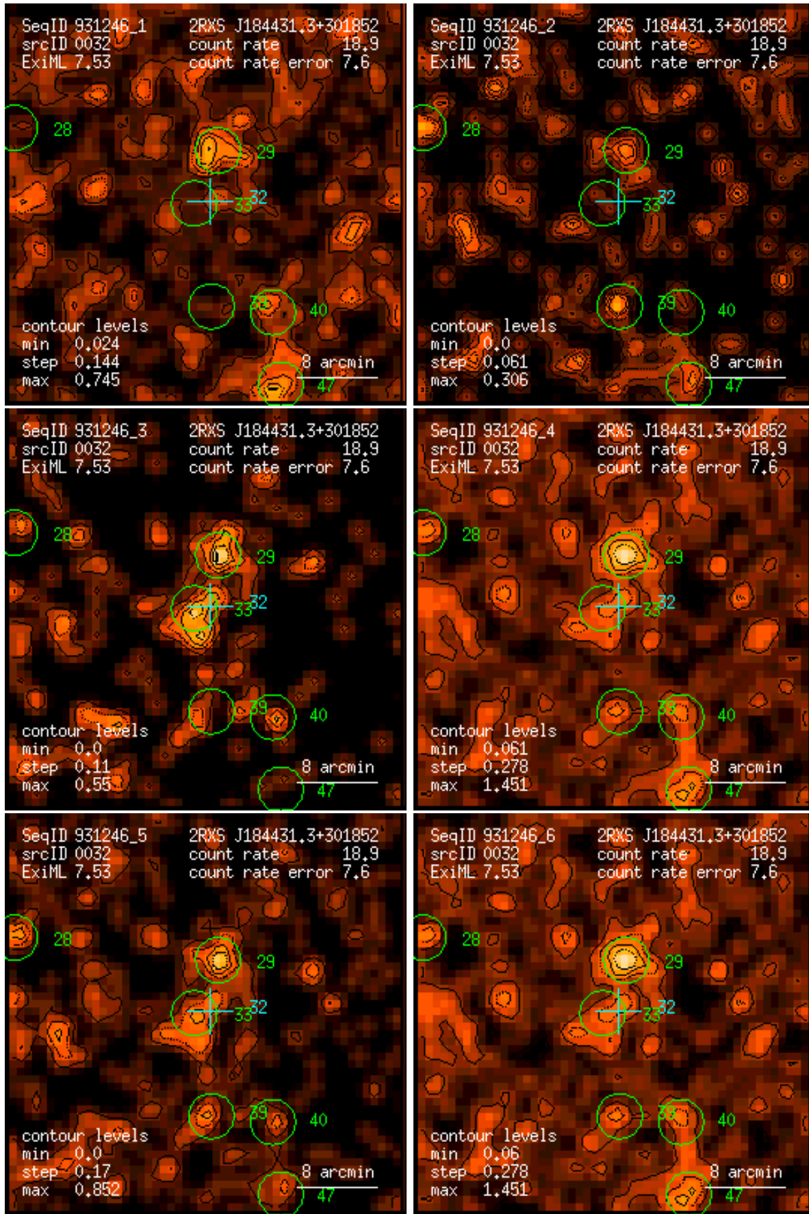
Figure 32: RASS 931246: detection 0032: band rate images, Gaussian filter: (1) PSPC channels 11 – 41, (2) 52 – 90, (3) 91 – 201, (4) 11 – 235, (5) 52 – 201, (6) 11 – 201. Broad band rates in counts/ks. Band rate contour levels in counts/ks/arcmin 2 .
