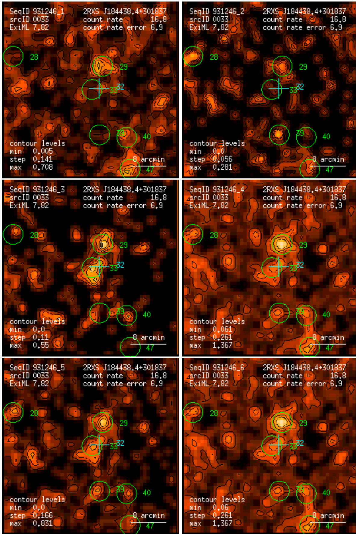
Figure 33: RASS 931246: detection 0033: band rate images, Gaussian filter: (1) PSPC channels 11 – 41, (2) 52 – 90, (3) 91 – 201, (4) 11 – 235, (5) 52 – 201, (6) 11 – 201. Broad band rates in counts/ks. Band rate contour levels in counts/ks/arcmin 2 .
