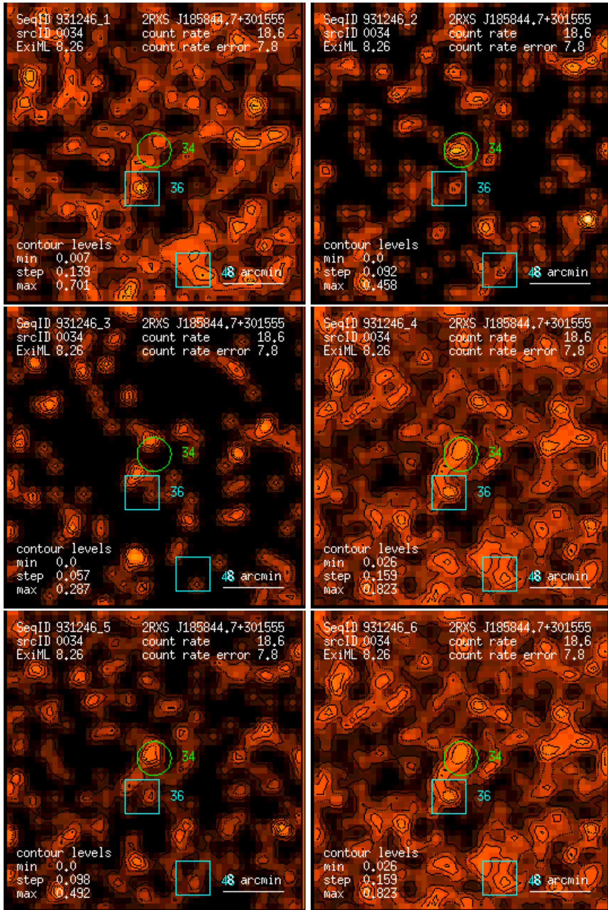
Figure 34: RASS 931246: detection 0034: band rate images, Gaussian filter: (1) PSPC channels 11 – 41, (2) 52 – 90, (3) 91 – 201, (4) 11 – 235, (5) 52 – 201, (6) 11 – 201. Broad band rates in counts/ks. Band rate contour levels in counts/ks/arcmin 2 .
