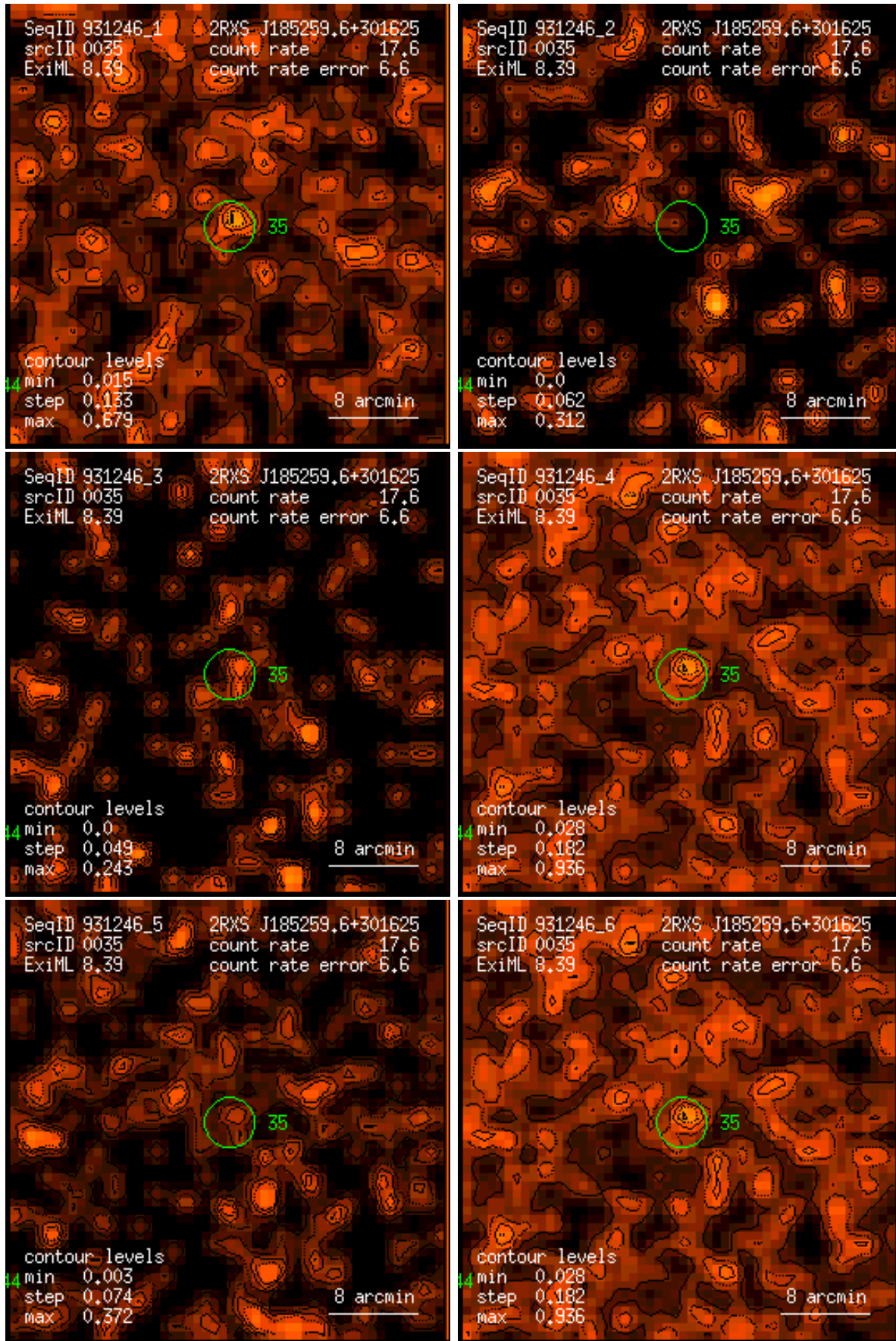
Figure 35: RASS 931246: detection 0035: band rate images, Gaussian filter: (1) PSPC channels 11 – 41, (2) 52 – 90, (3) 91 – 201, (4) 11 – 235, (5) 52 – 201, (6) 11 – 201. Broad band rates in counts/ks. Band rate contour levels in counts/ks/arcmin 2 .
