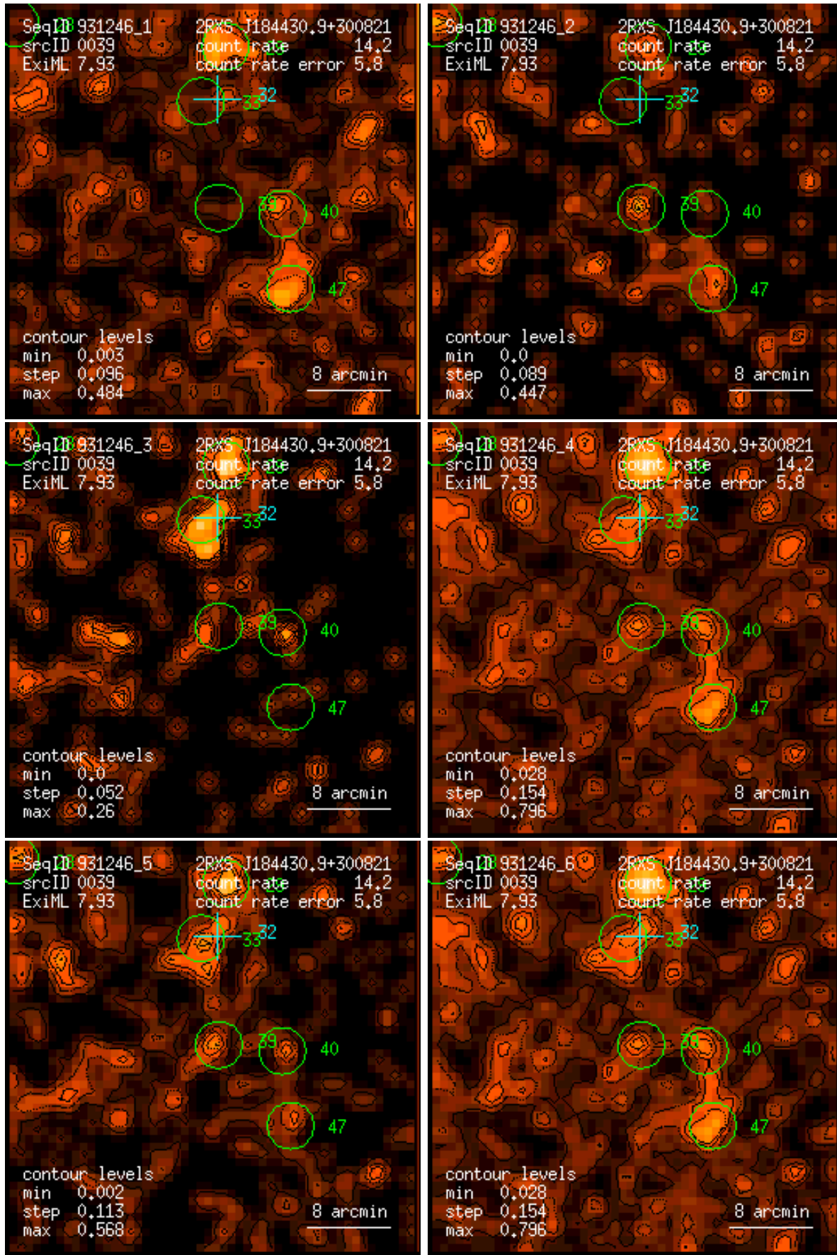
Figure 39: RASS 931246: detection 0039: band rate images, Gaussian filter: (1) PSPC channels 11 – 41, (2) 52 – 90, (3) 91 – 201, (4) 11 – 235, (5) 52 – 201, (6) 11 – 201. Broad band rates in counts/ks. Band rate contour levels in counts/ks/arcmin 2 .
