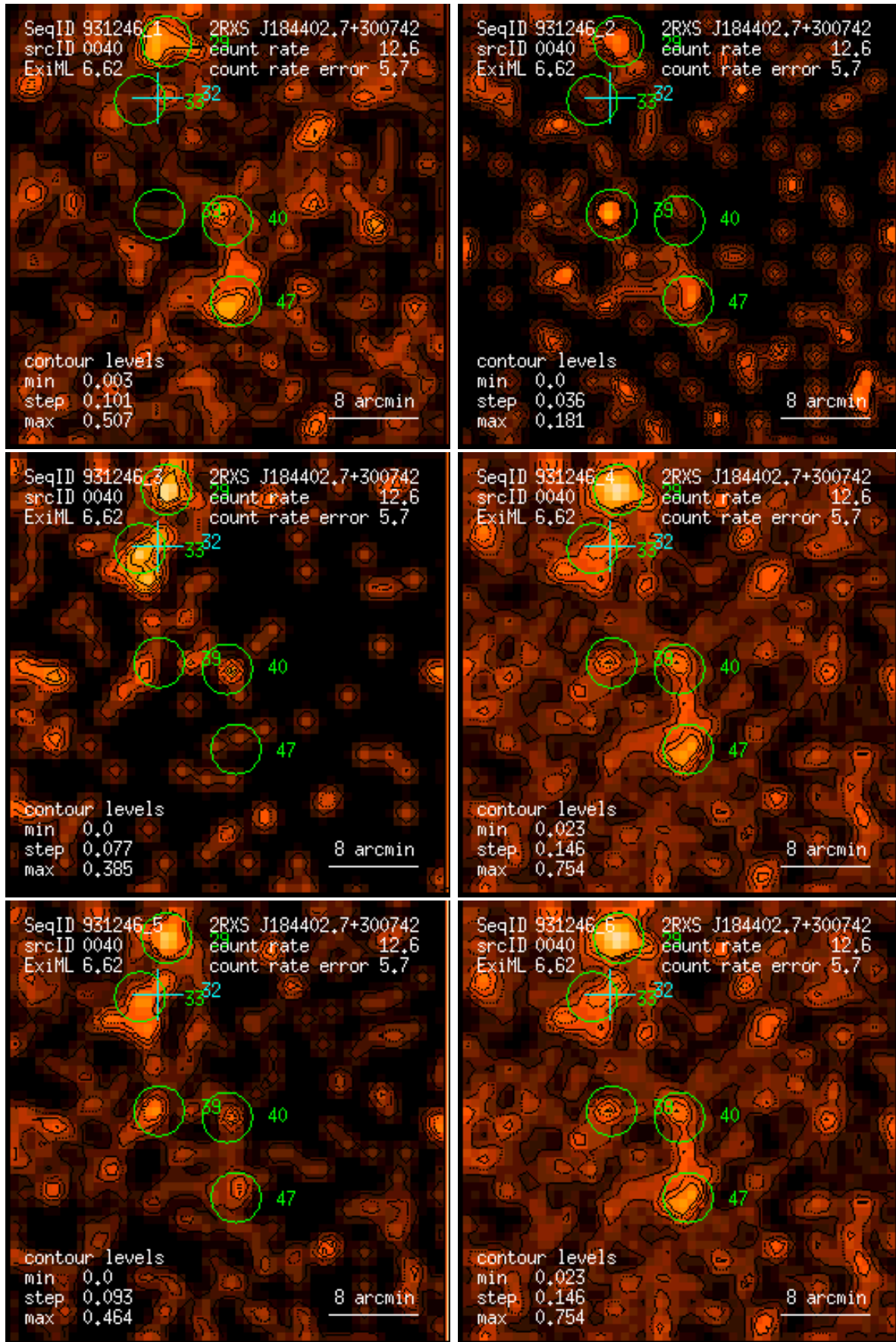
Figure 40: RASS 931246: detection 0040: band rate images, Gaussian filter: (1) PSPC channels 11 – 41, (2) 52 – 90, (3) 91 – 201, (4) 11 – 235, (5) 52 – 201, (6) 11 – 201. Broad band rates in counts/ks. Band rate contour levels in counts/ks/arcmin 2 .
