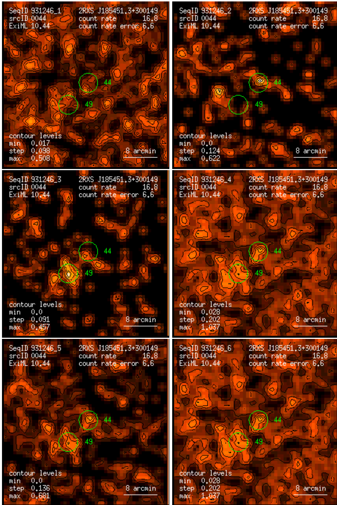
Figure 44: RASS 931246: detection 0044: band rate images, Gaussian filter: (1) PSPC channels 11 – 41, (2) 52 – 90, (3) 91 – 201, (4) 11 – 235, (5) 52 – 201, (6) 11 – 201. Broad band rates in counts/ks. Band rate contour levels in counts/ks/arcmin 2 .
